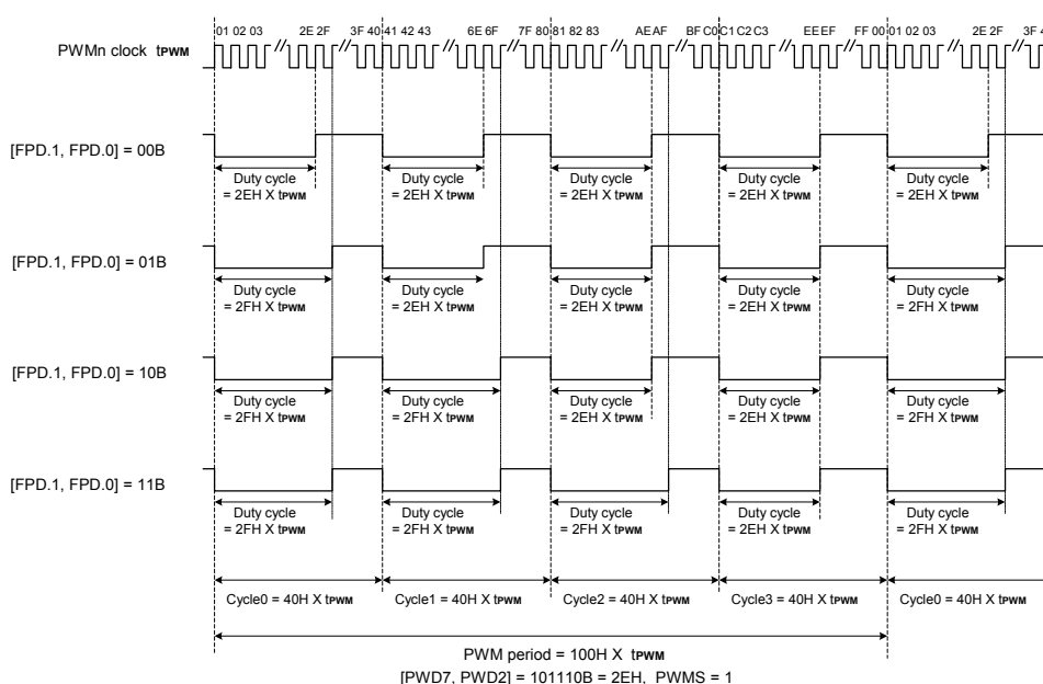
Figure 4. PWM Output Example in Negative Mode
