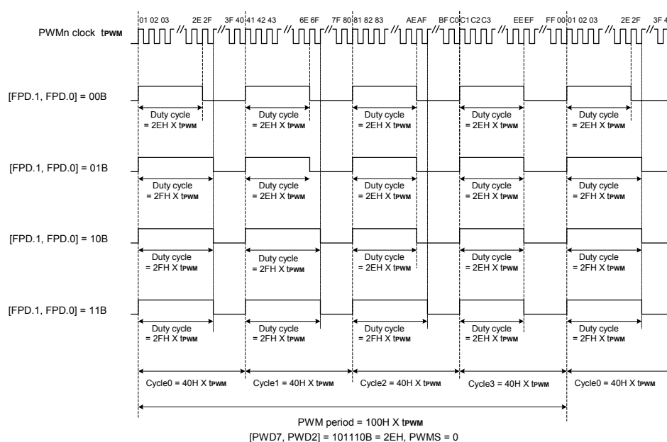
Figure 3. PWM Output Example in Normal Mode
