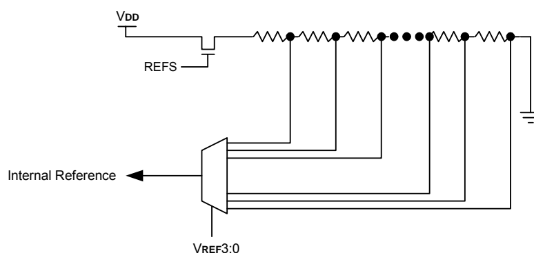
Figure 6. Comparator Internal Reference Block Diagram
