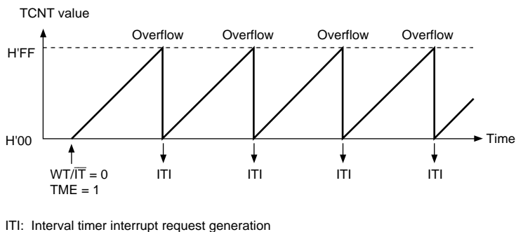
Figure 12.3 Operation in Interval Timer Mode
