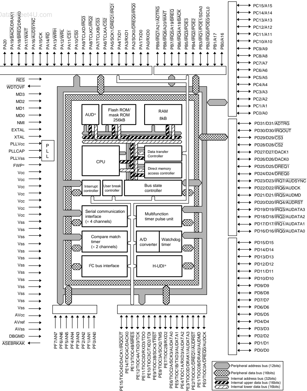
Figure 1.2 Block Diagram of SH7145
