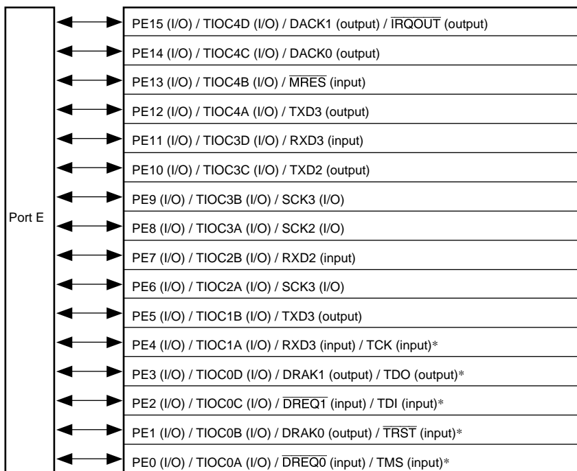
Figure 18.7 Port E (SH7144)
