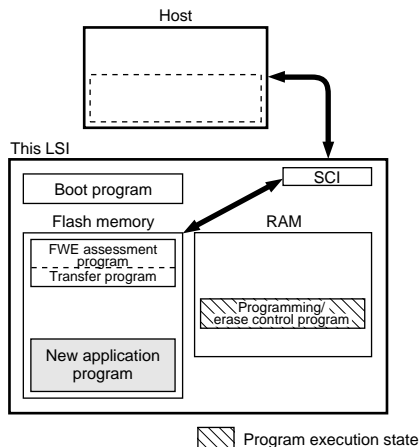
Figure 19.4 User Program Mode
