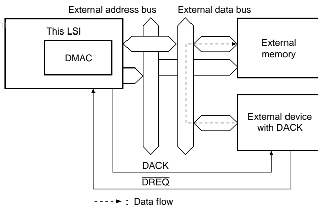
Figure 10.4 Data Flow in Single Address Mode
