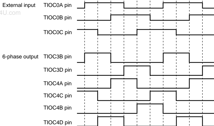
Figure 11.50 Example of Output Phase Switching by External Input (1)
