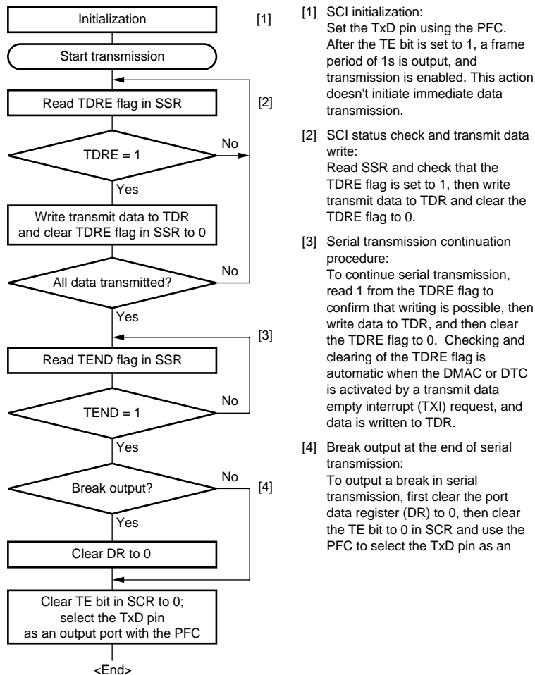
Figure 13.7 Sample Serial Transmission Flowchart
