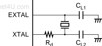
Figure 4.2 Connection of the Crystal Oscillator (Example)
