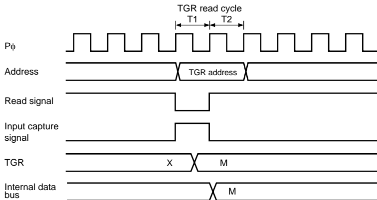
Figure 11.76 Contention between TGR Read and Input Capture
