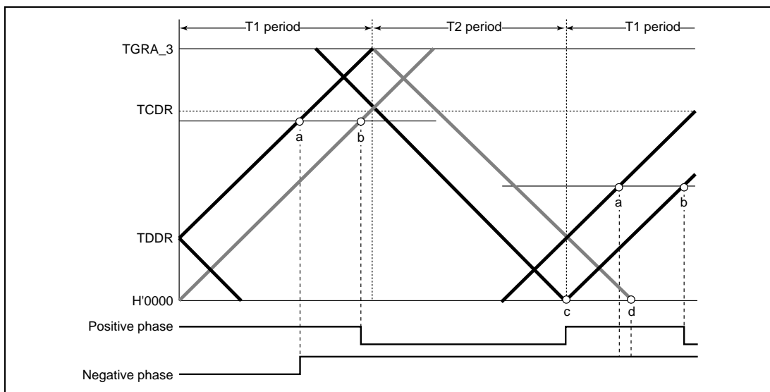
Figure 11.44 Example of Complementary PWM Mode 0% and 100% Waveform Output (2)
