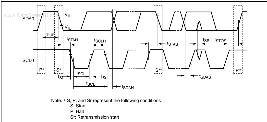
Figure 26.21 I²C Bus Interface Timing
