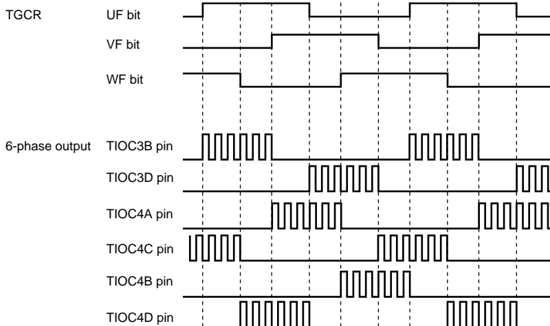
Figure 11.53 Example of Output Phase Switching by Means of UF, VF, WF Bit Settings (2)
