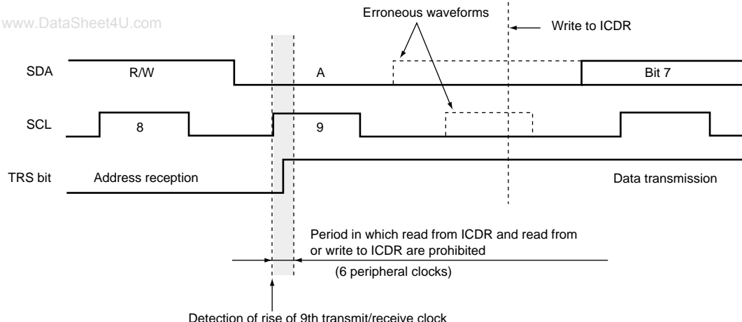
Figure 14.21 Scheme of Slave Transmit Operation
