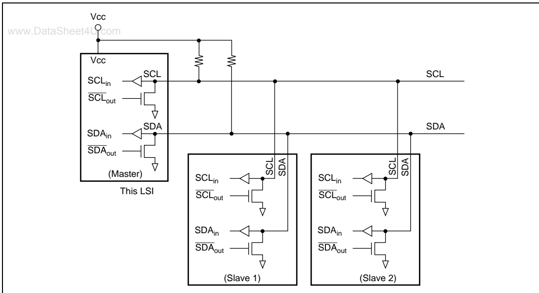
Figure 14.2 Example of the Connection of I²C Bus Interfaces (This LSI is the Master Device)
