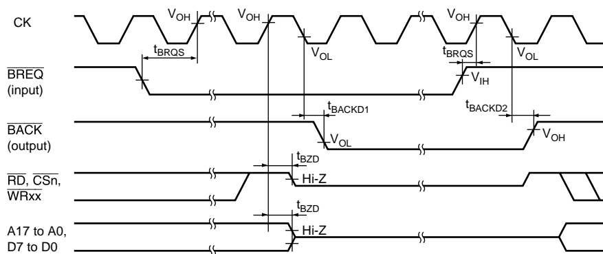
Figure 26.8 Bus Release Timing
