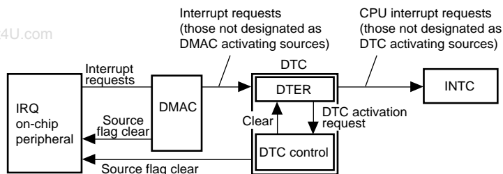
Figure 8.2 Activating Source Control Block Diagram
