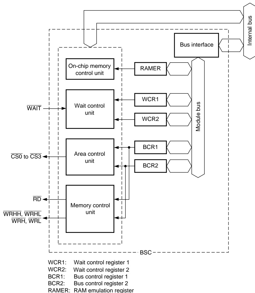
Figure 9.1 BSC Block Diagram
