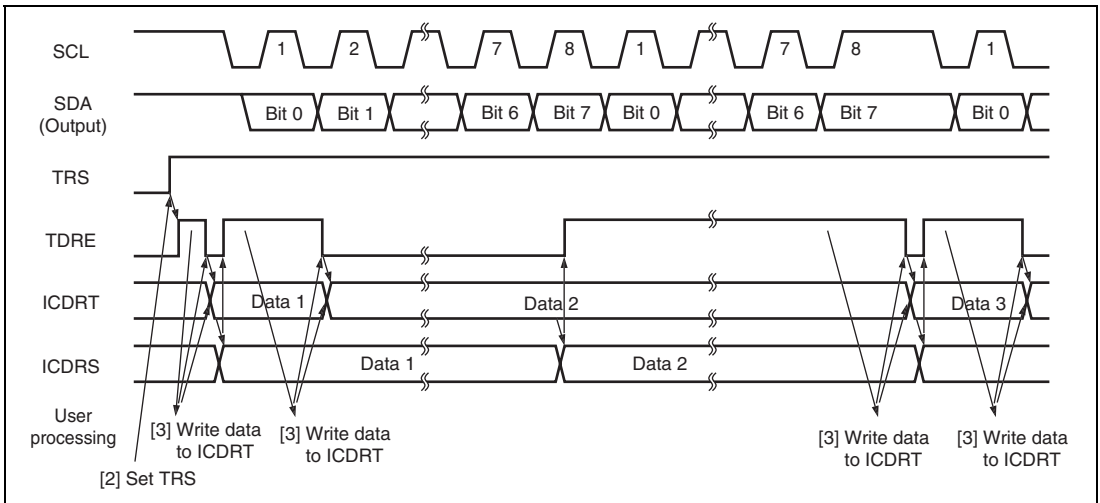
Figure 20.14 Transmit Mode Operation Timing
