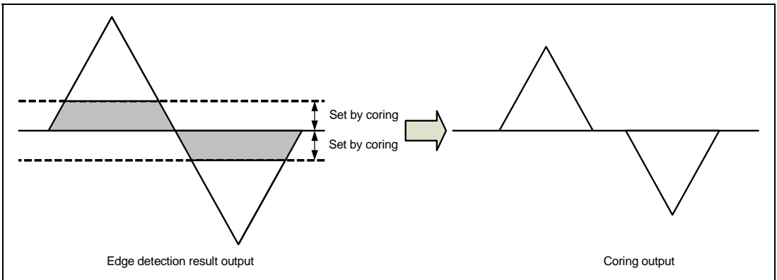
Figure 34.5 LTI Coring
