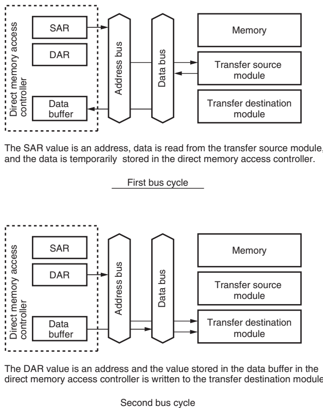
Figure 11.3 Data Flow of Dual Address Mode
