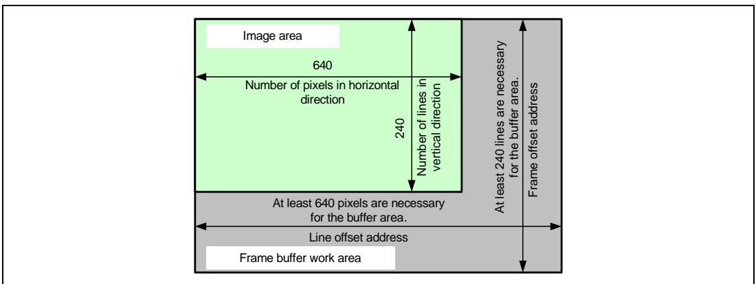
Figure 33.19 Frame Buffer Access Area Setting
