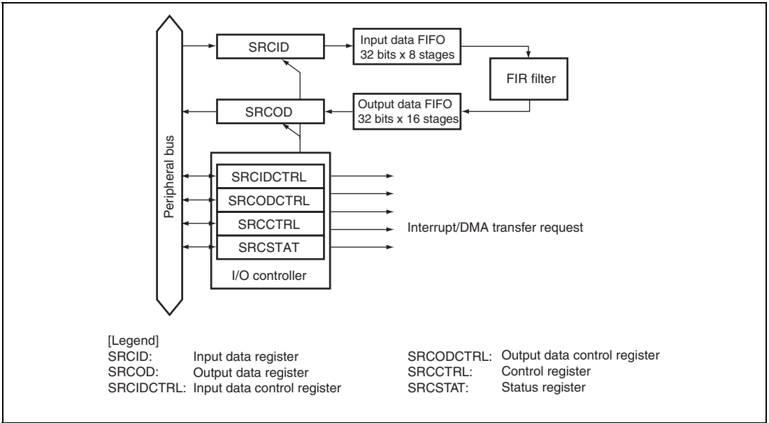
Figure 42.1 Block Diagram
