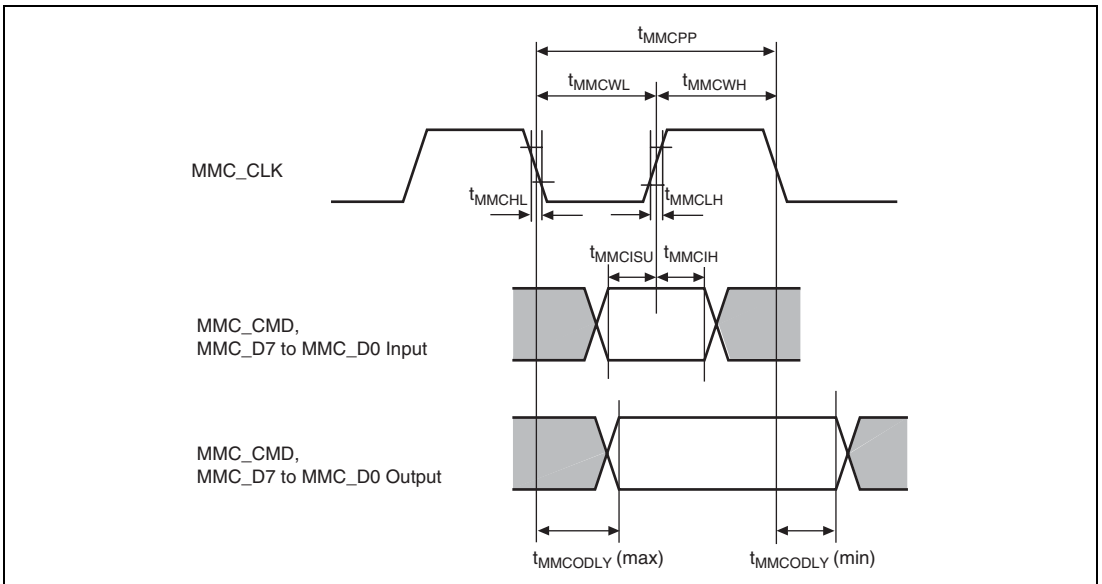
Figure 52.82 MMC Interface
