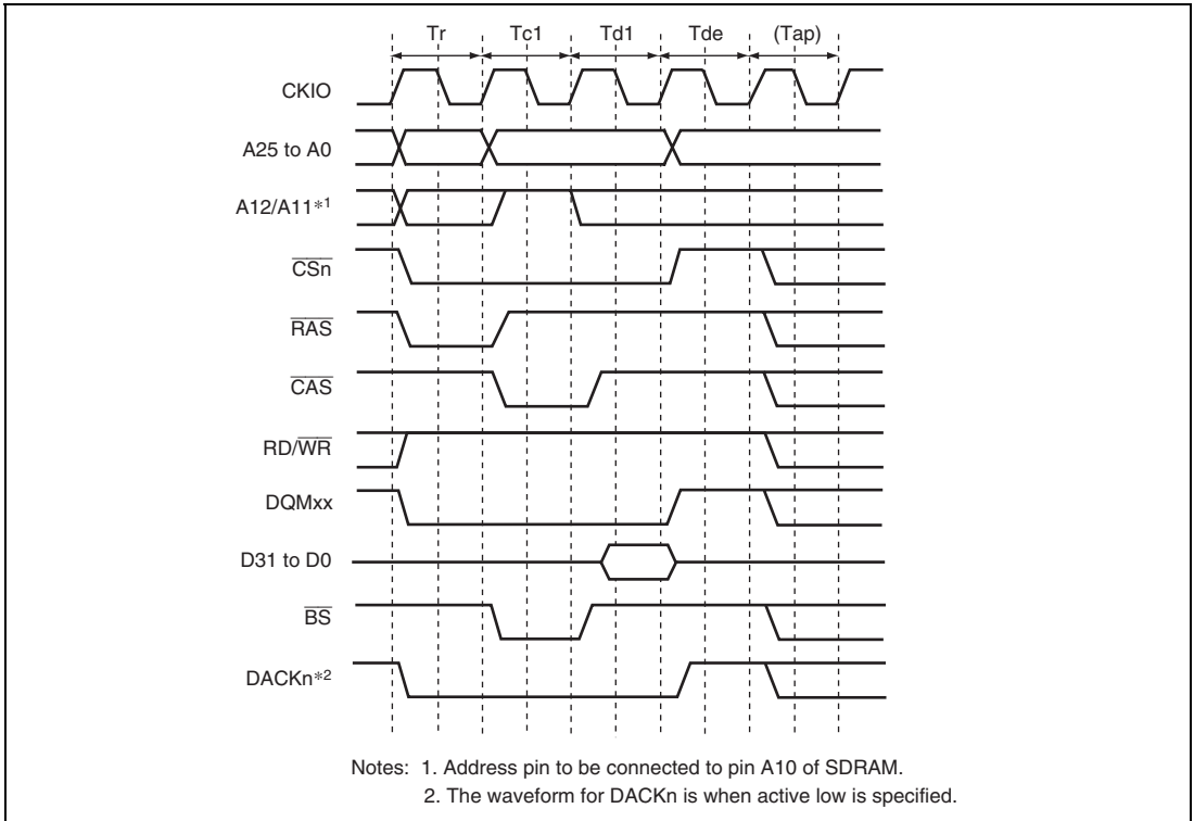
Figure 10.18 Basic Timing for Single Read (CAS Latency 1, Auto Pre-Charge)
