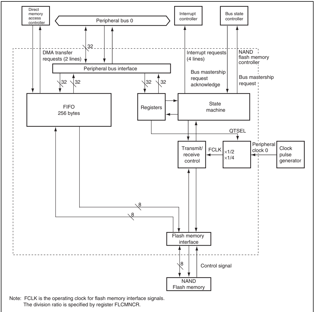
Figure 28.1 Block Diagram
