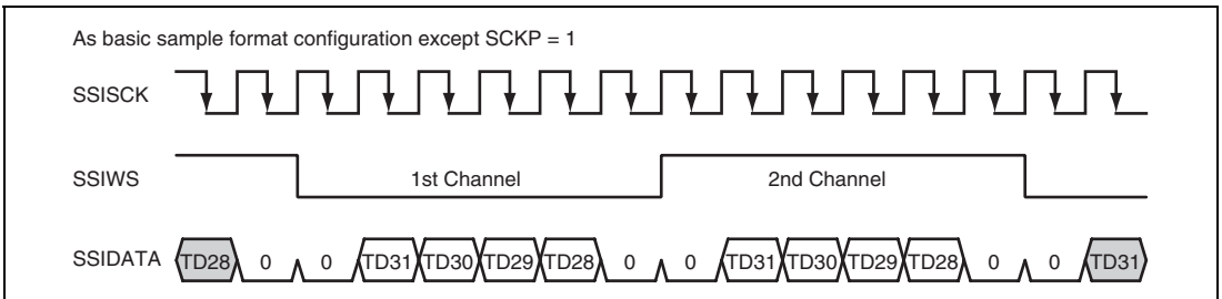
Figure 21.10 Inverted Clock
