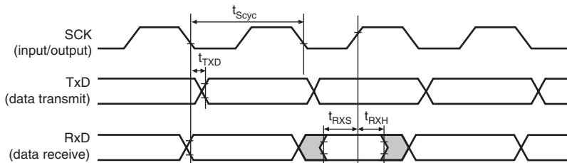
Figure 52.44 Transmit/Receive Data Input/Output Timing in Clocked Synchronous Mode
