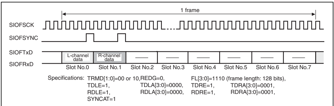
Figure 22.15 Transmit and Receive Timing (16-Bit Stereo Data)
