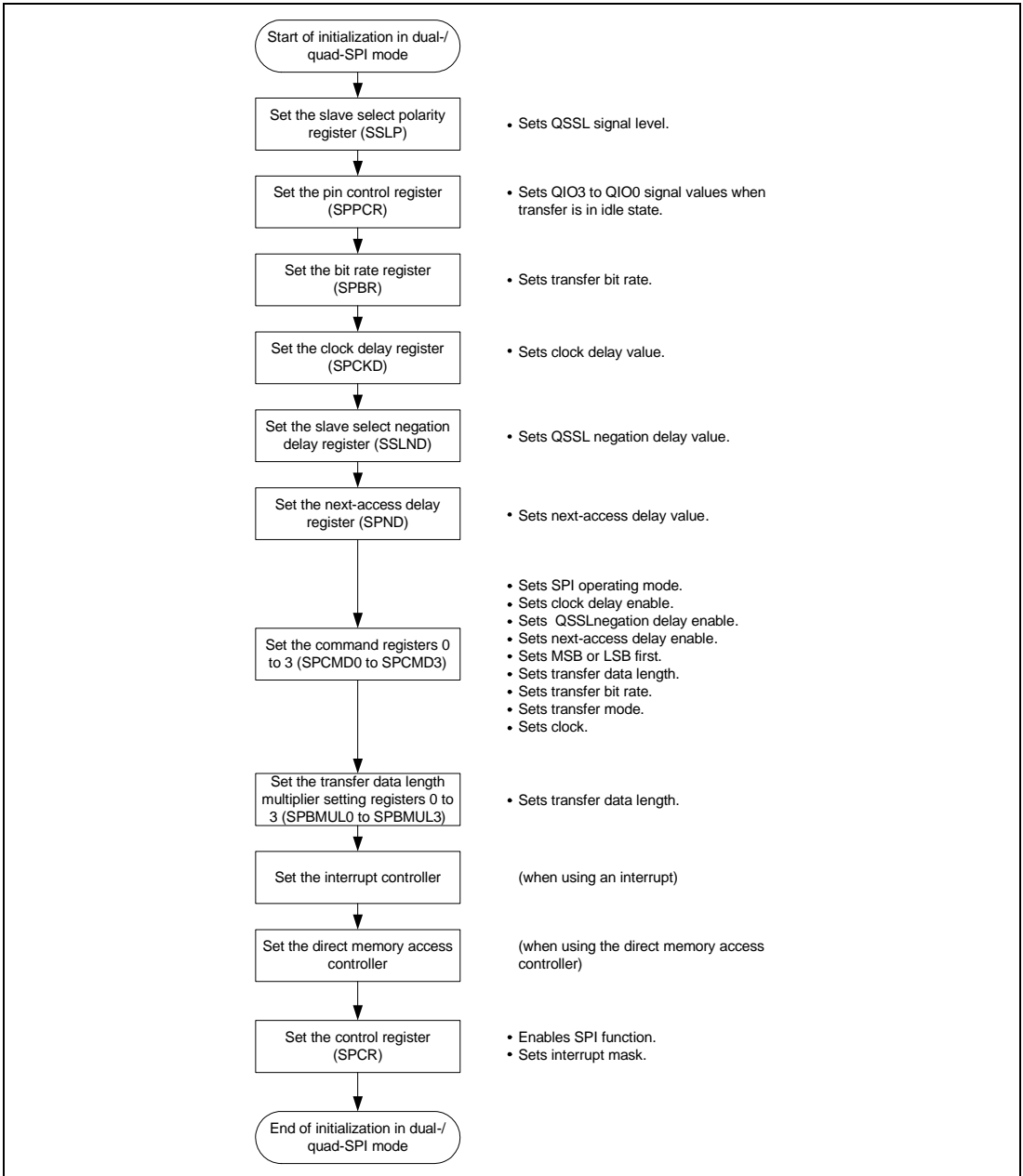
Figure 18.20 Example of Initialization Flowchart in Dual-/Quad-SPI Mode
