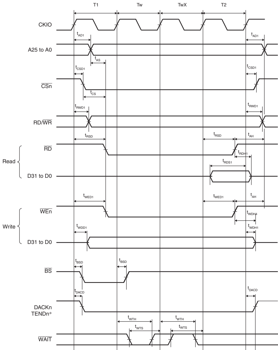
Figure 52.11 Basic Bus Timing for Normal Space (One Software Wait Cycle, One External Wait Cycle)
