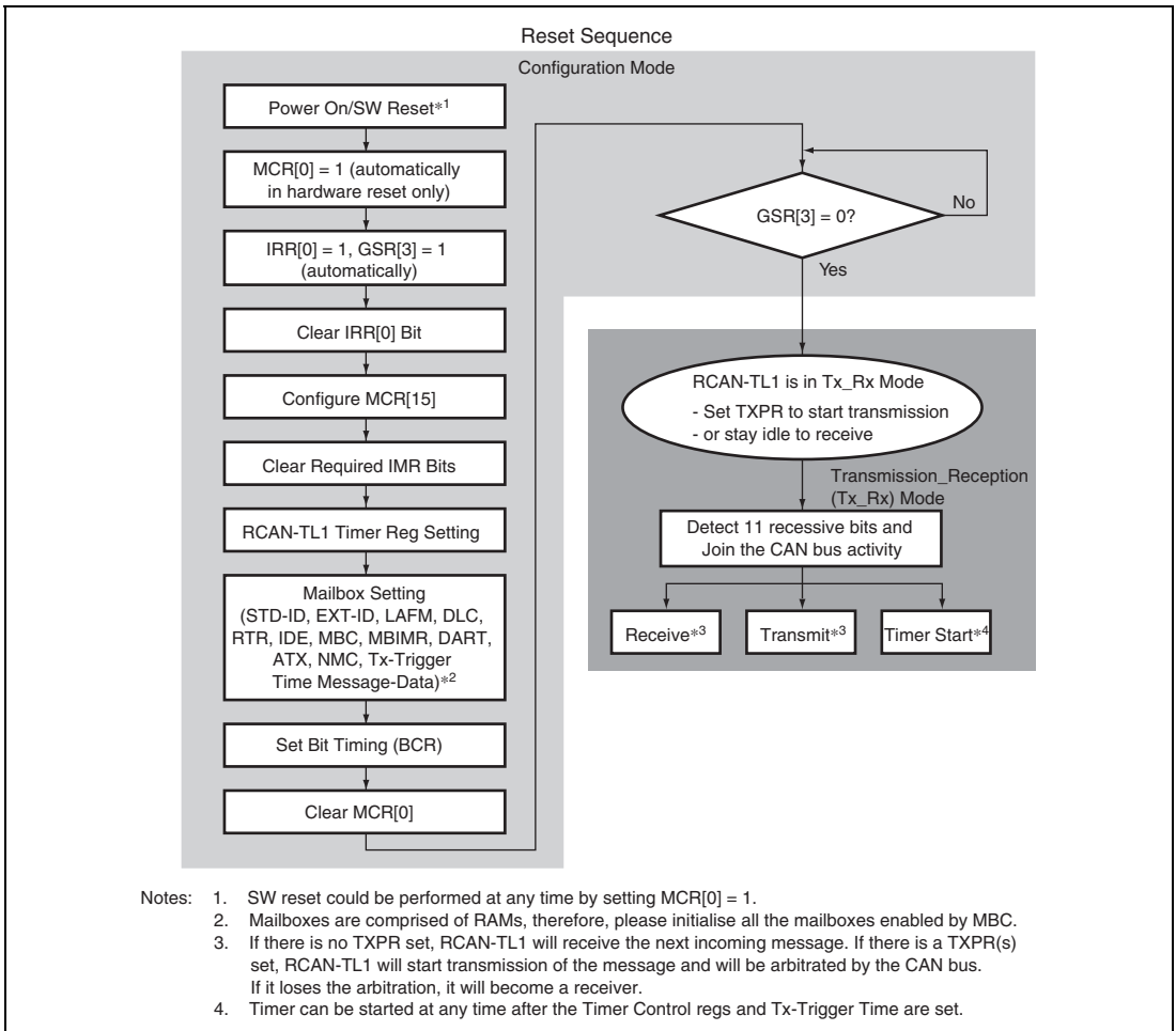
Figure 23.14 Reset Sequence
