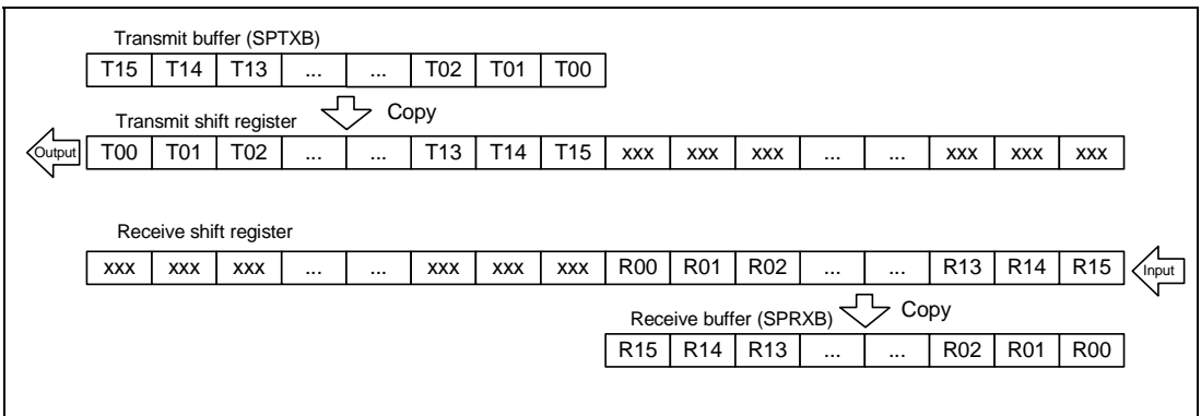
Figure 18.9 LSB First Transfer (16-Bit Data)
