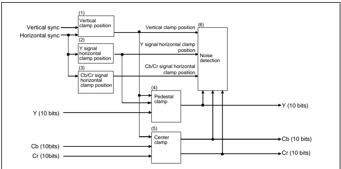
Figure 30.37 Block Diagram of Digital Clamp Circuit
