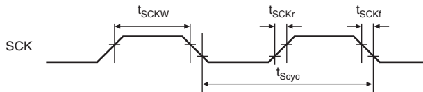
Figure 52.43 SCK Input Clock Timing
