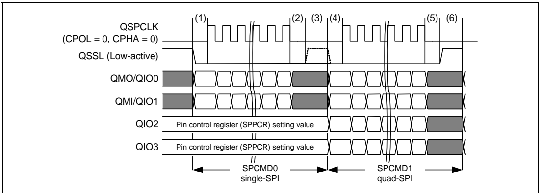
Figure 18.19 Burst Transfer Example in which QSSL Signal Level Keeping Function is Used (Single- and Quad-SPI Modes Used)
