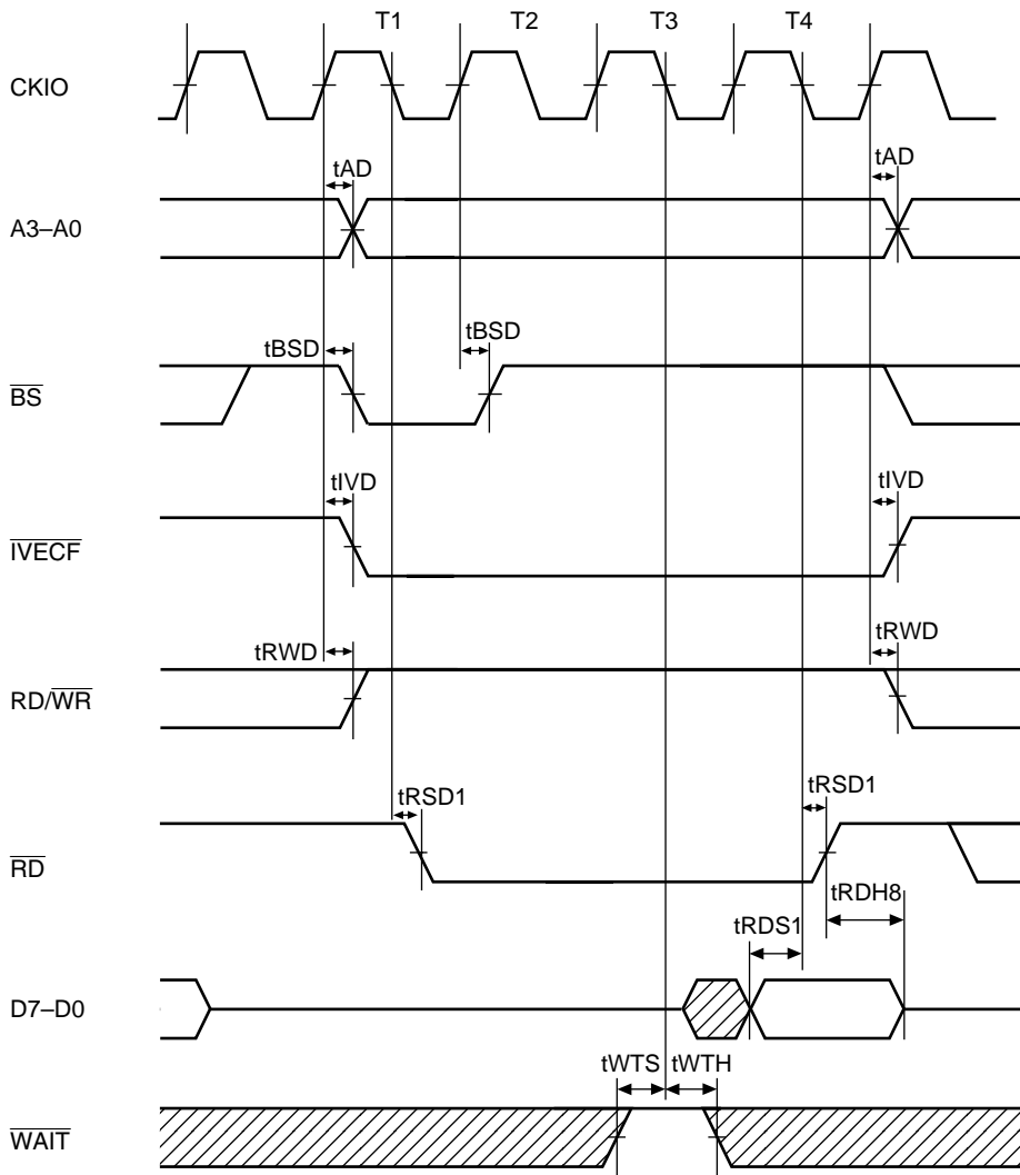
Figure 21.43 Interrupt Vector Fetch Cycle (No Wait, I\phi:E\phi = 1:1 )
