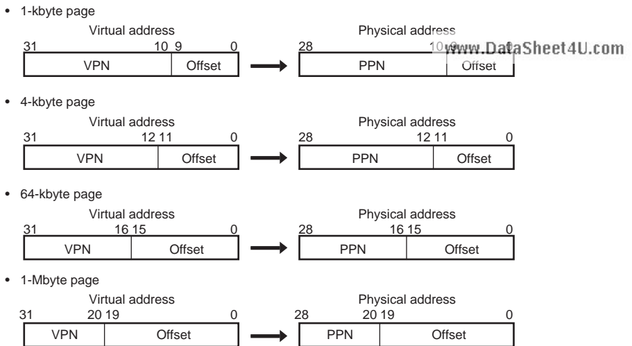
Figure 6.7 Relationship between Page Size and Address Format
