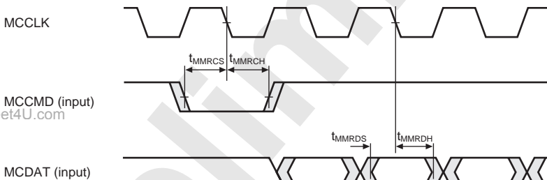
Figure 33.78 MMCIF Receive Timing (falling edge sampling)
