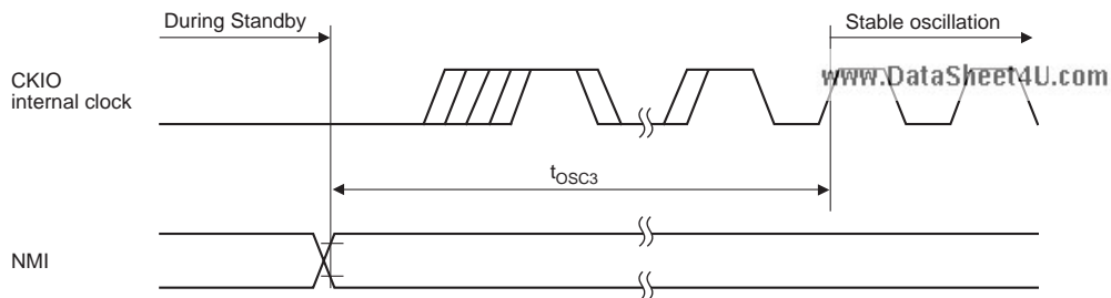
Figure 33.10 Standby Return Oscillation Settling Time (Return by NMI)
