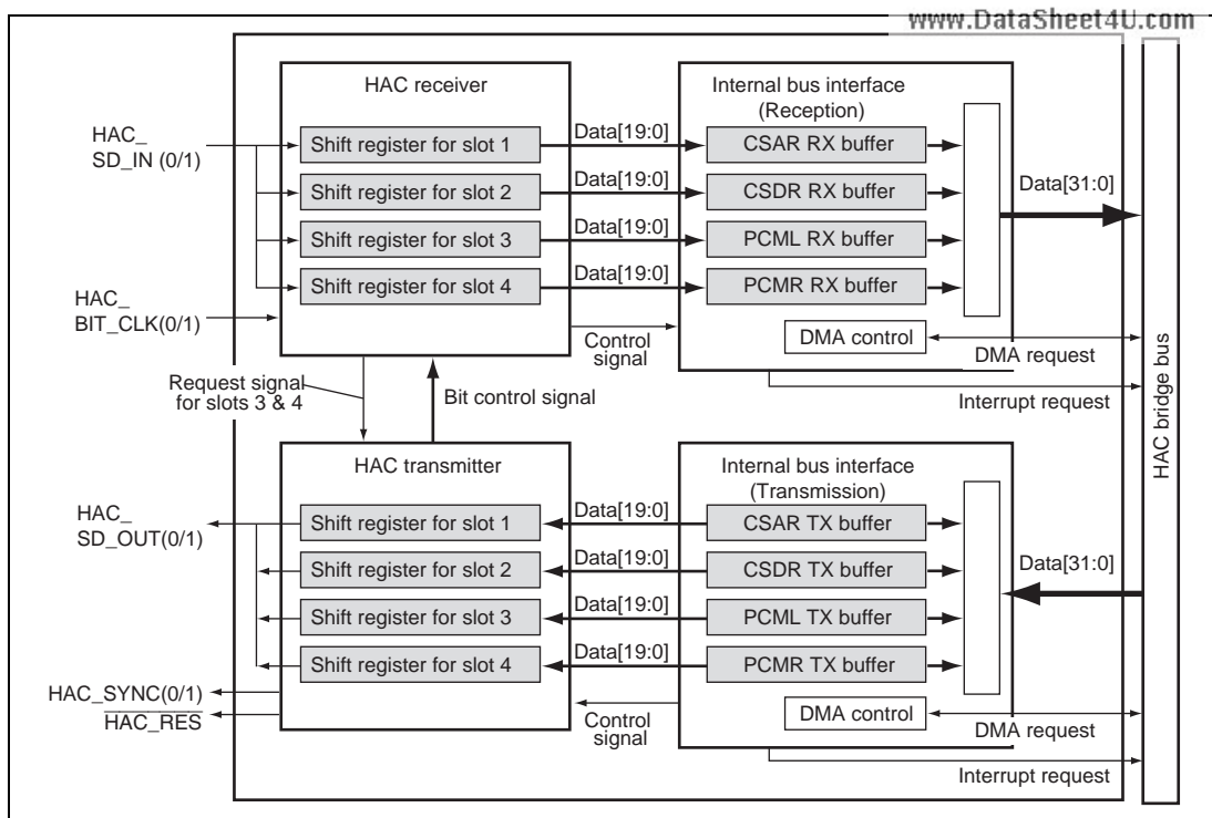
Figure 25.1 Block Diagram
