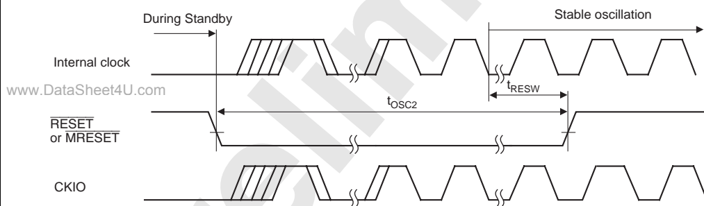
Figure 33.8 Power-On Oscillation Settling Time (2)
