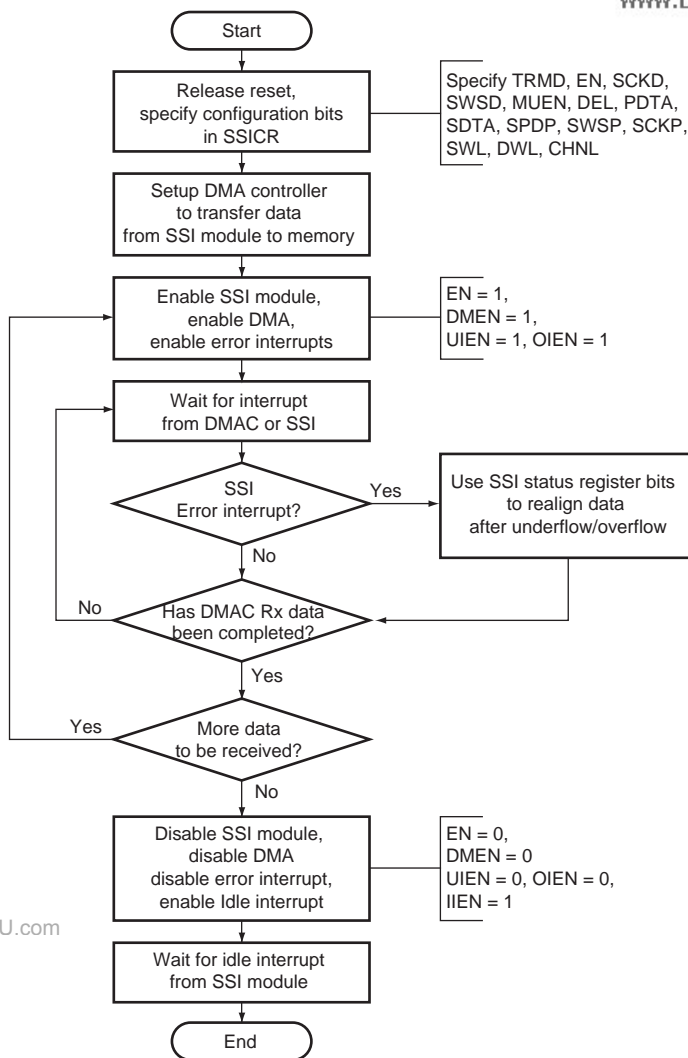
Figure 20.23 Reception using DMA Controller
