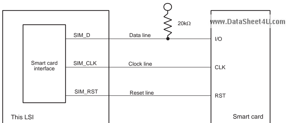
Figure 18.12 Example of Smart Card Interface Pin Connections
