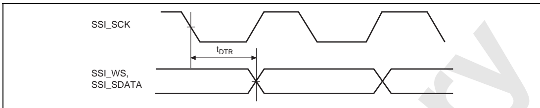
Figure 33.86 SSI Transmit Timing
