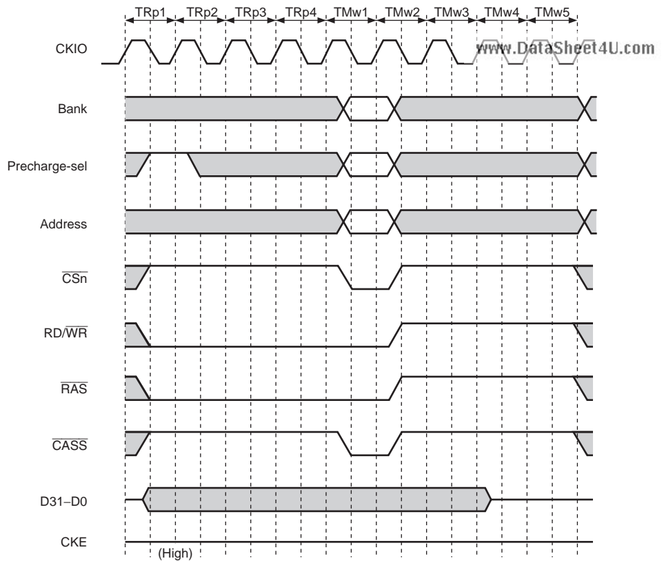
Figure 10.30(2) Synchronous DRAM Mode Write Timing (Mode Register Setting)
