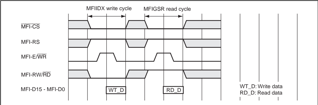
Figure 27.6 Writing to MFIIIDX and Reading from MFIGSR
