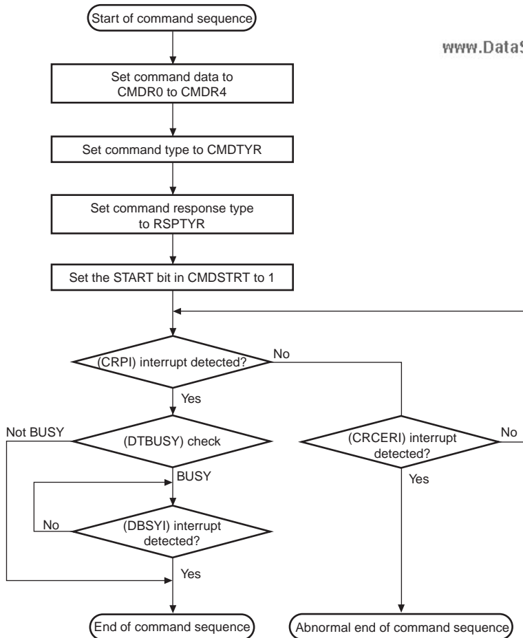
Figure 26.7 Example of Operational Flow for Commands without Data Transfer
