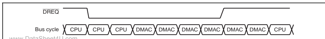
Figure 11.11 Example of DMA Transfer in Burst Mode
