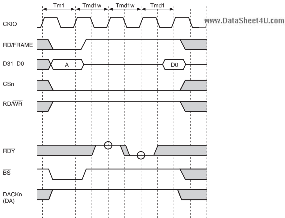
Figure 10.45 MPX Interface Timing 2 (Single Read, AnW = 0, One External Wait Inserted)
