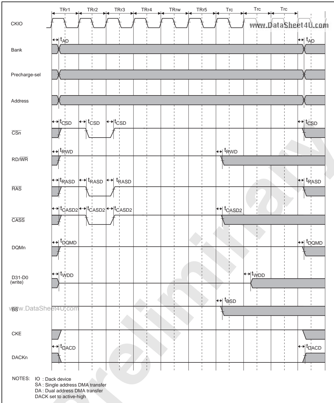
Figure 33.36 Synchronous DRAM Bus Cycle: Auto-Refresh (TRAS=1, TRC[2:0]=001)
