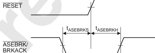
Figure 33.55 \overline{\text{RESET}} Hold Timing
