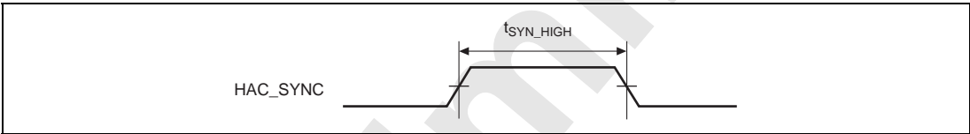
Figure 33.81 HAC Cold Reset Timing
