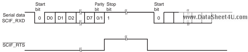
Figure 17.14 Sample Operation Using Modem Control ( \overline{\text{SCIF\_RTS}} ) (Only in Channels 1 and 2)
