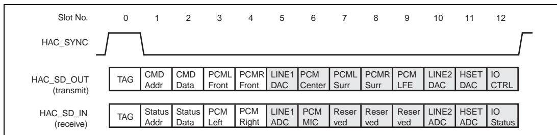
Figure 25.2 AC97 Frame Slot Structure
