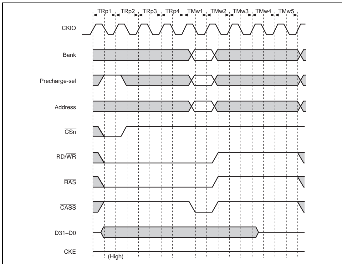
Figure 10.30(1) Synchronous DRAM Mode Write Timing (PALL)
