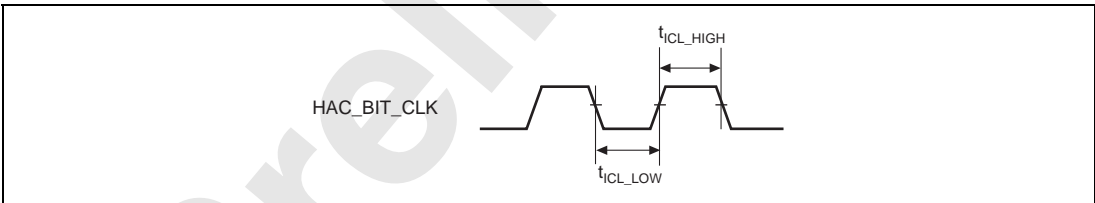
Figure 33.82 HAC Clock Input Timing
