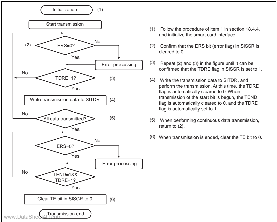
Figure 18.5 Example of Transmission Processing
