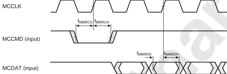
Figure 33.77 MMCIF Receive Timing (rising edge sampling)
