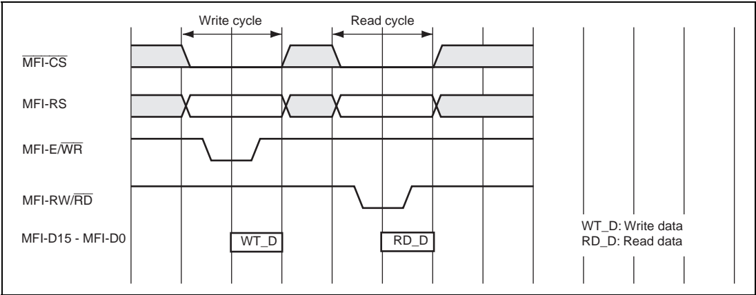
Figure 27.5 Basic Timing of the MFI 80-Series Interface
