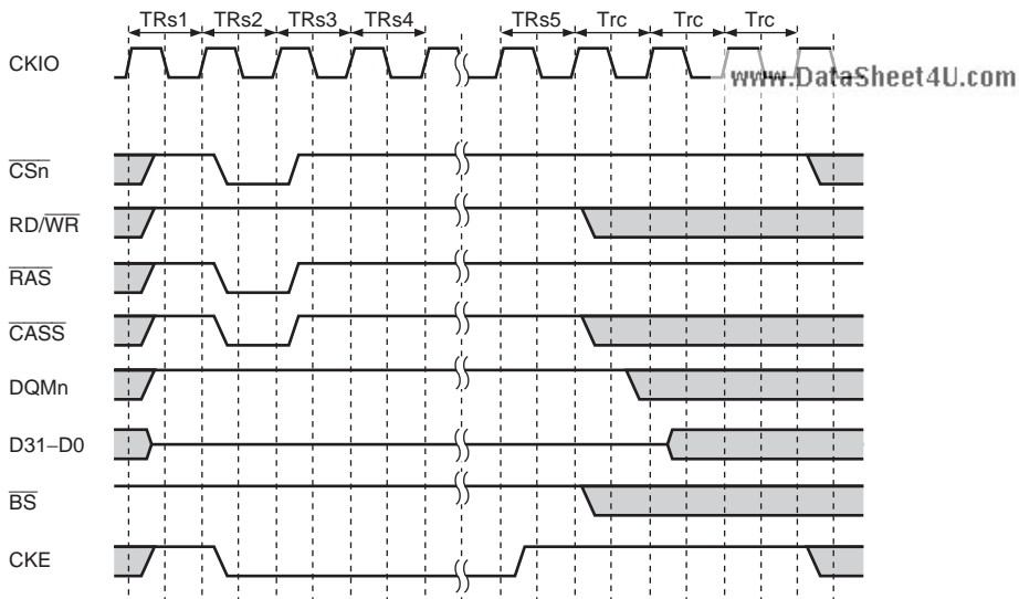
Figure 10.29 Synchronous DRAM Self-Refresh Timing
