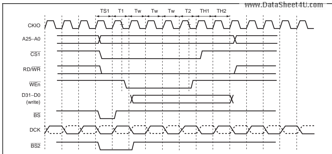
Figure 10.14 DCK, \overline{\text{BS2}} , and \overline{\text{CS1}} Timing when Writing to SRAM Interface (DCKDR = H'0002, A1RDH = 1 and A1H[1:0] = 10 in WCR3, CSH[1:0] in WCR4 = 10, Three Wait Cycles)
