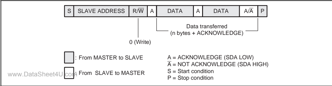
Figure 19.3 Master Data Transmit format
