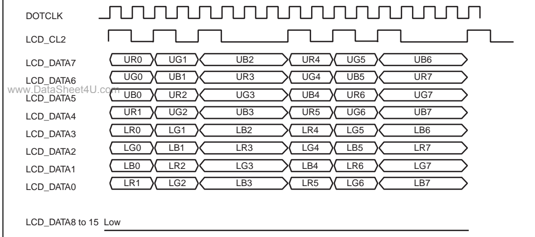
Figure 30.16 Clock and LCD Data Signal Example
