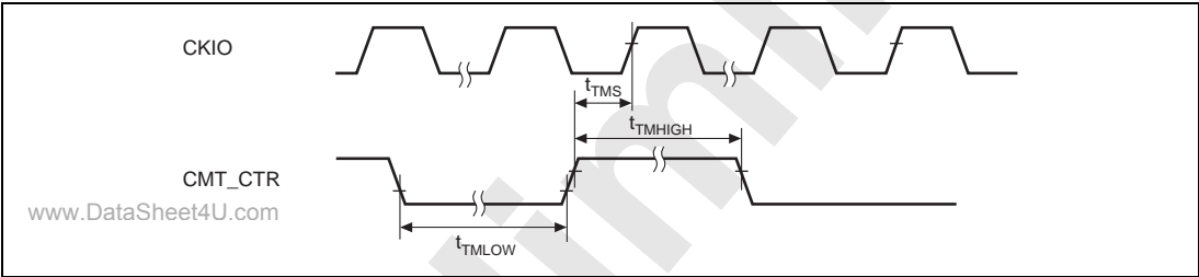
Figure 33.59 CMT Timing (2)
