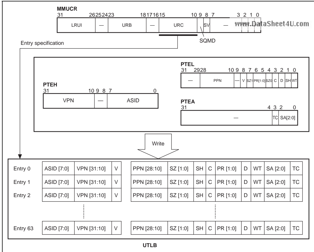
Figure 6.11 Operation of LDTLB Instruction
