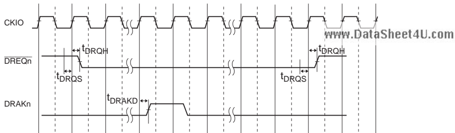
Figure 33.50 \overline{\text{DREQ}}/\text{DRAK} Timing
