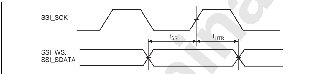
Figure 33.87 SSI Receive Timing (1)
