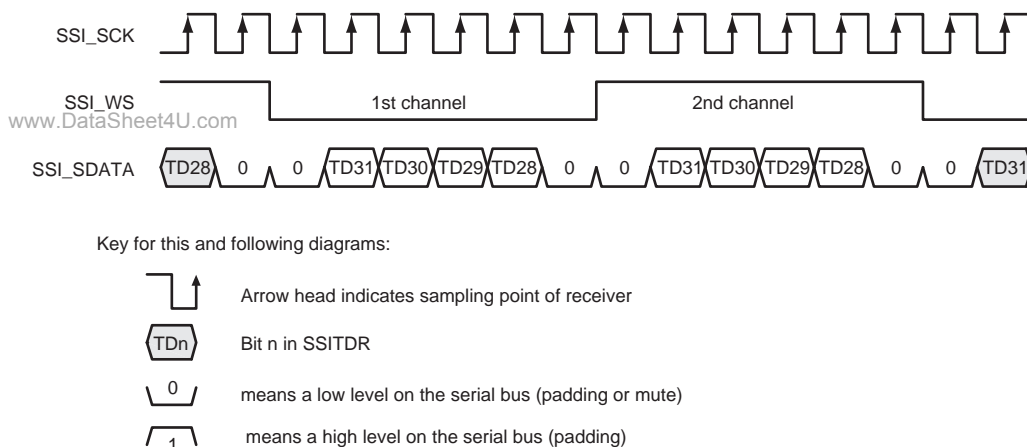
Figure 20.9 Basic Sample Format (Transmit Mode with Example System/Data Word Length)
