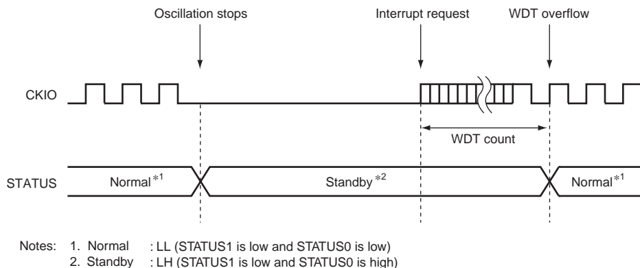
Figure 14.3 STATUS Output in Sequence of Software Standby → Interrupt
