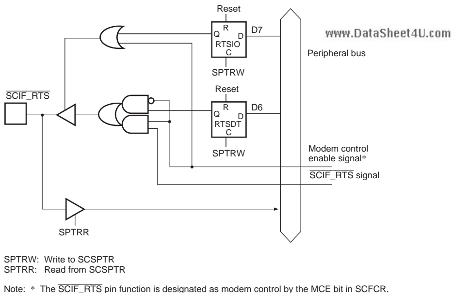
Figure 17.2 SCIF_RTS Pin (Only in Channels 1 and 2)
