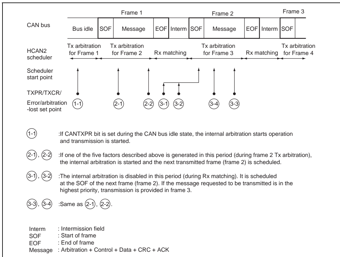
www.DataSheet4U.com Figure 22.7 Internal Arbitration for Transmission
