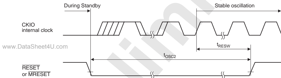
Figure 33.6 Power-On Oscillation Settling Time (1)
