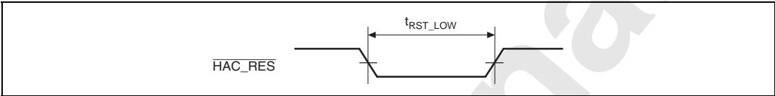
Figure 33.80 HAC Cold Reset Timing
