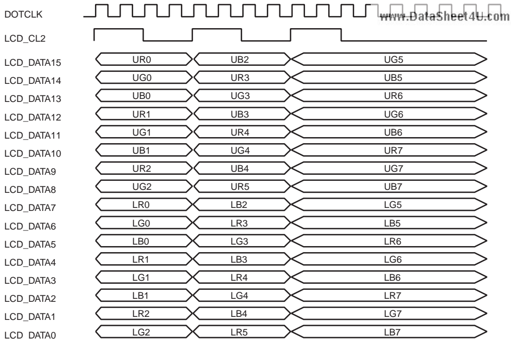
Figure 30.18 Clock and LCD Data Signal Example
