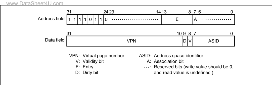
Figure 6.15 Memory-Mapped UTLB Address Array
