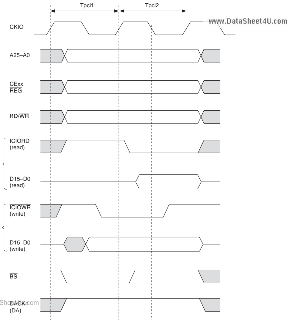
Figure 10.40 Basic Timing for PCMCIA I/O Card Interface
