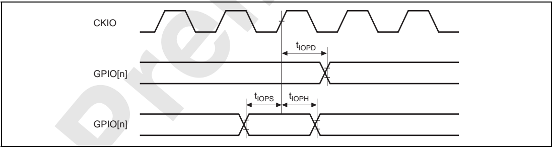
Figure 33.61 GPIO Timing
