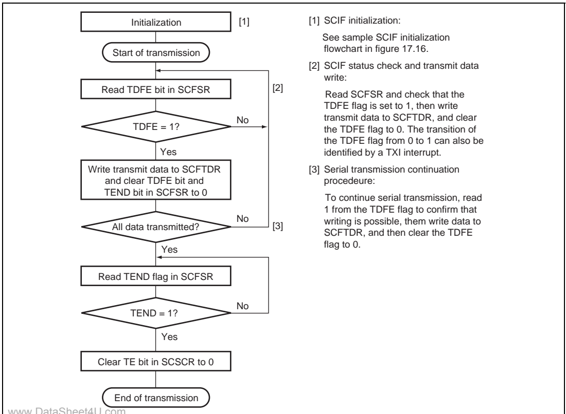
Figure 17.17 Sample Serial Transmission Flowchart
