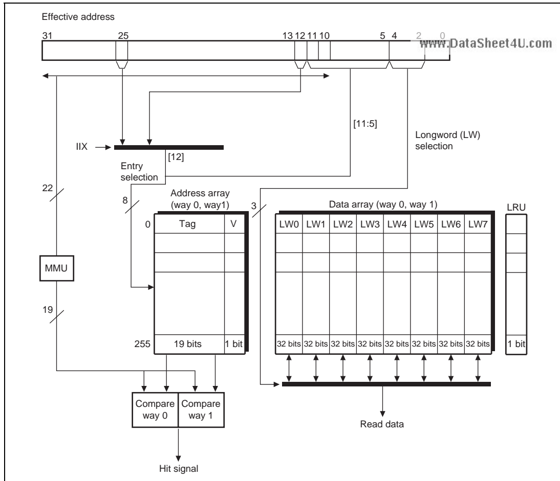
Figure 7.2 Configuration of Instruction Cache
