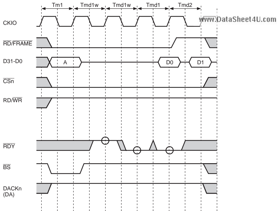
Figure 10.53 MPX Interface Timing 10 (Burst Read Cycle, AnW = 0, One External Wait Inserted, 32-Bit Bus Width, 64-Bit Data Transfer)
