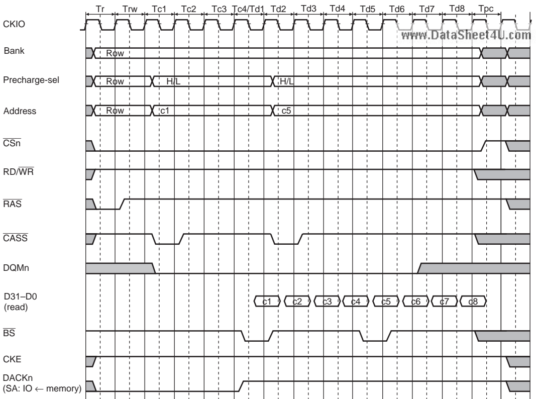
Figure 10.16 Basic Timing for Synchronous DRAM Burst Read
