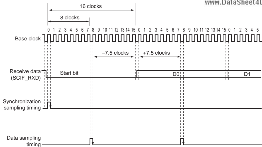
Figure 17.22 Receive Data Sampling Timing in Asynchronous Mode
