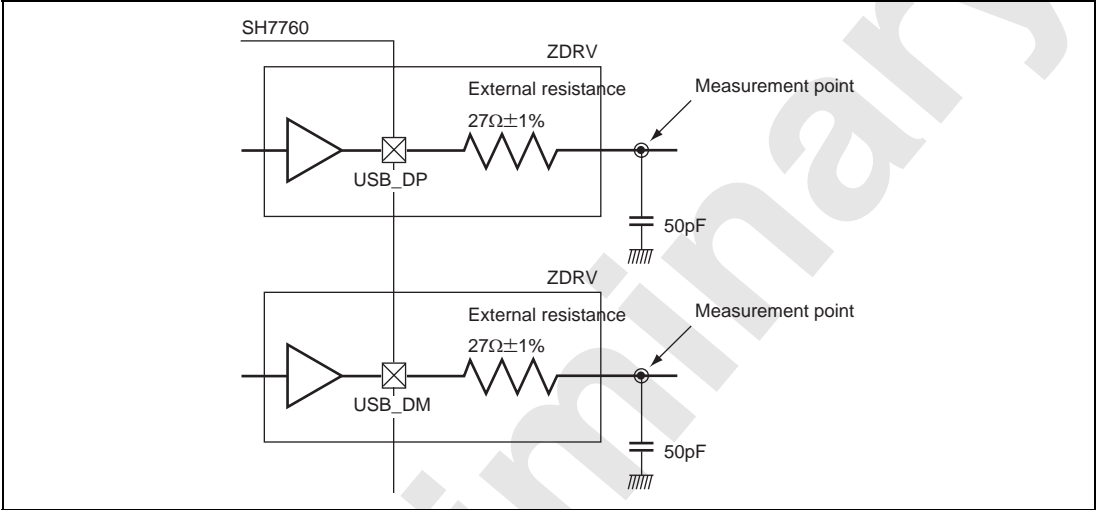
www.DataSheet4U.com Figure 33.68 Load Condition of AC Characteristics (Full speed)
