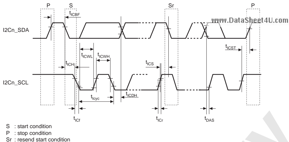
Figure 33.63 I 2 C Bus Interface Module Signal Timing
