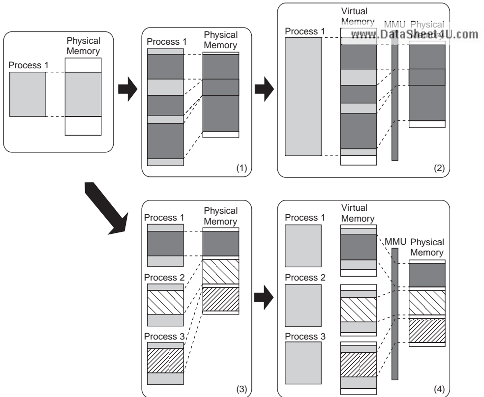
Figure 6.1 Role of the MMU
