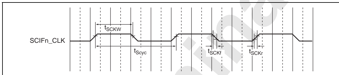
Figure 33.52 SCIFn_CLK Input Clock Timing
