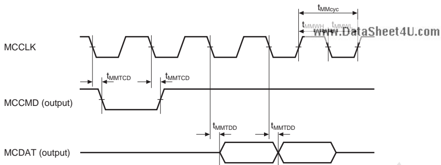
Figure 33.76 MMCIF Transmit Timing
