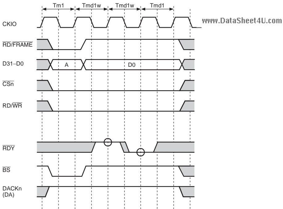
Figure 10.47 MPX Interface Timing 4 (Single Write, AnW = 1, One External Wait Inserted)
