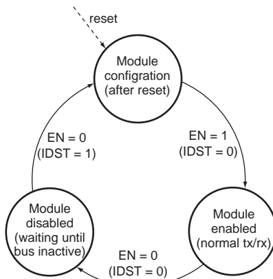
Figure 20.20 Transition Diagram between Operation Modes
