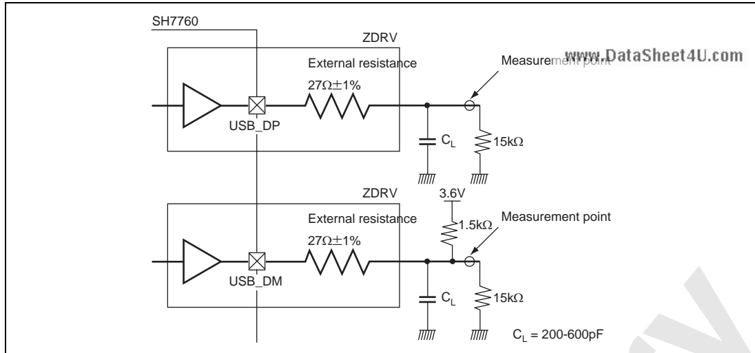
Figure 33.69 Load Condition of AC Characteristics (Low speed)
