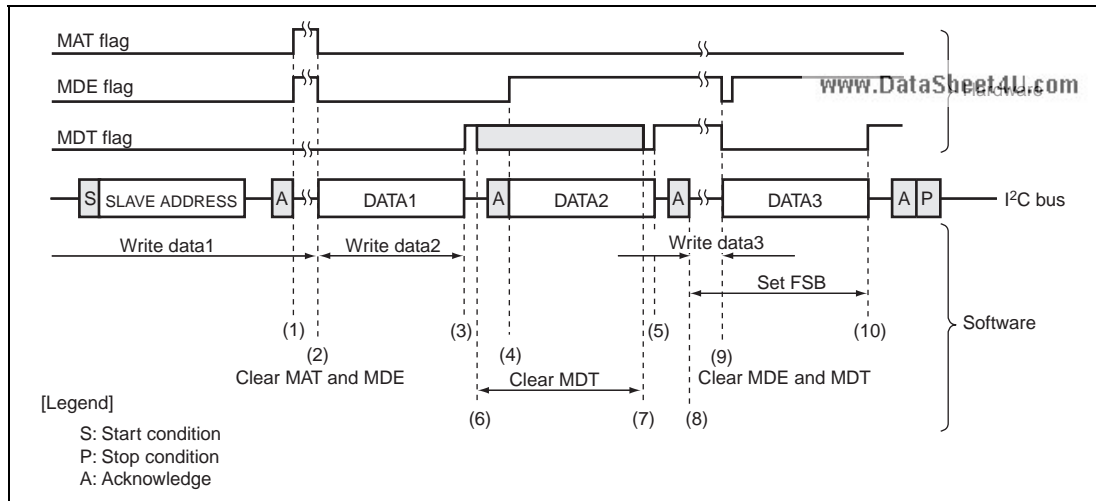
Figure 19.13 Operational Example of Three-byte Data Transmission
