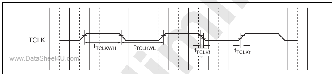
Figure 33.51 TCLK Input Timing
