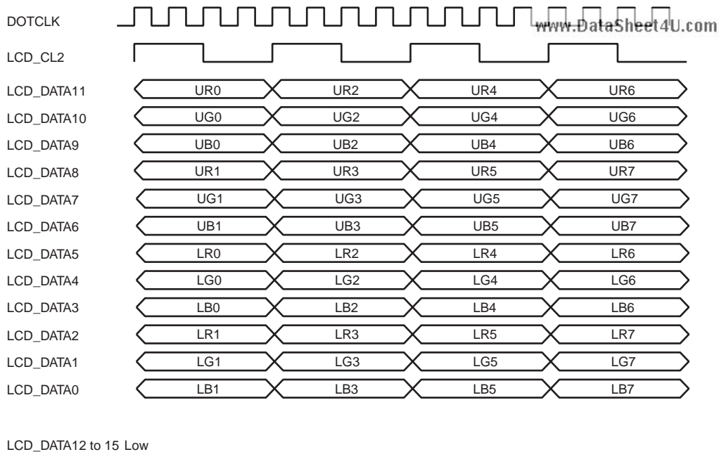
Figure 30.17 Clock and LCD Data Signal Example
