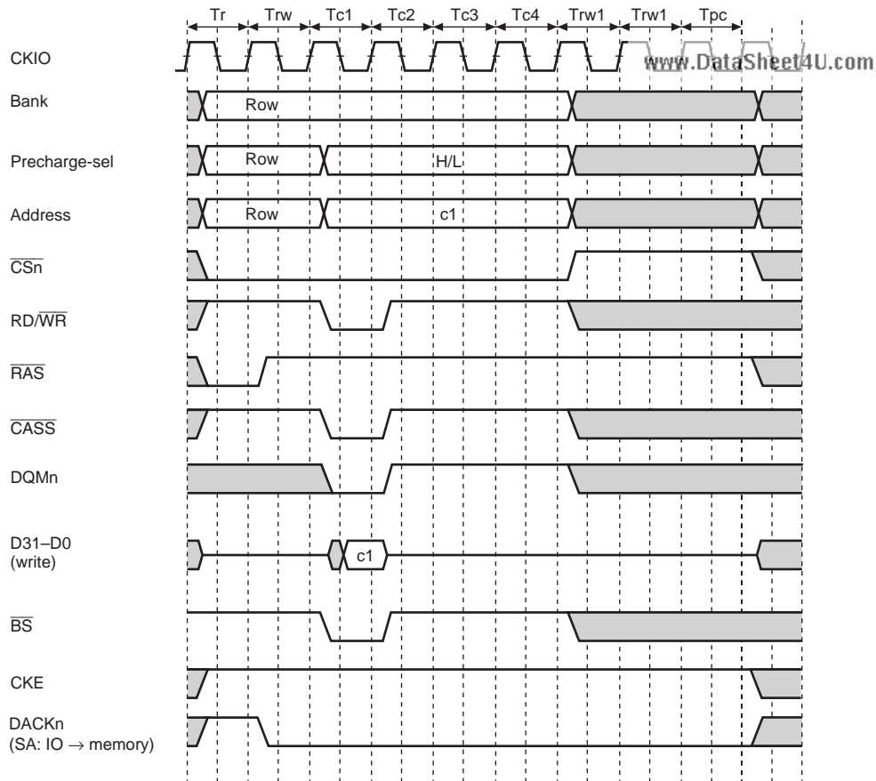
Figure 10.19 Basic Timing for Synchronous DRAM Single Write
