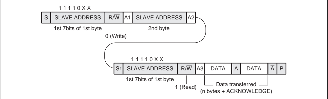
Figure 19.7 10-Bit Address Data Receive Format
