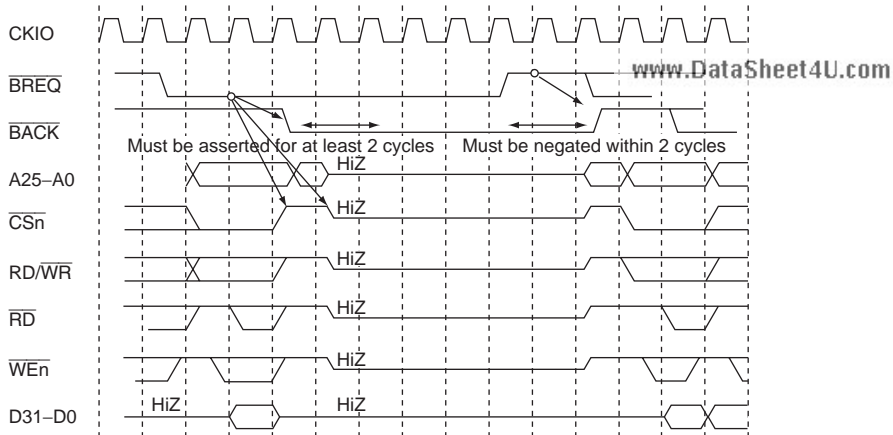
Figure 10.61 Arbitration Sequence
