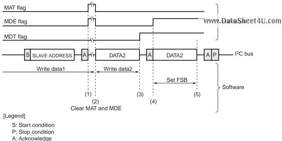
Figure 19.12 Operational Example of Two-byte Data Transmission
