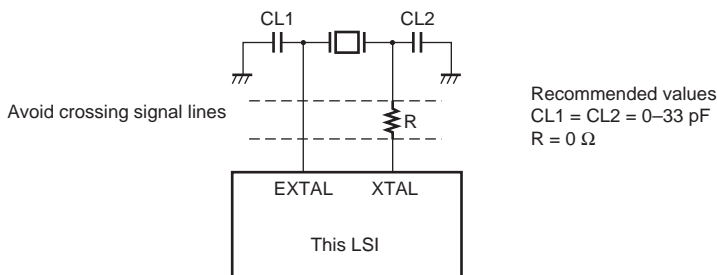
Figure 12.2 Points for Attention when Using Crystal Resonator
