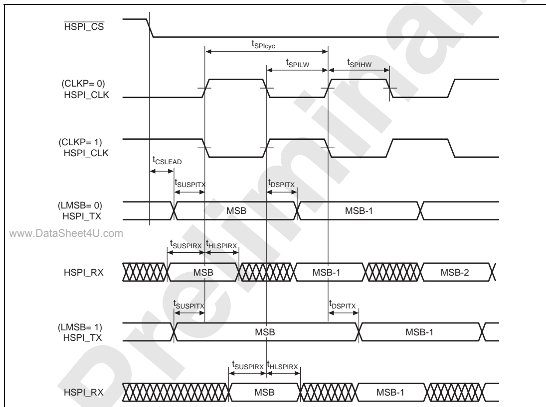
Figure 33.64 HSPI Data Output/Input Timing
