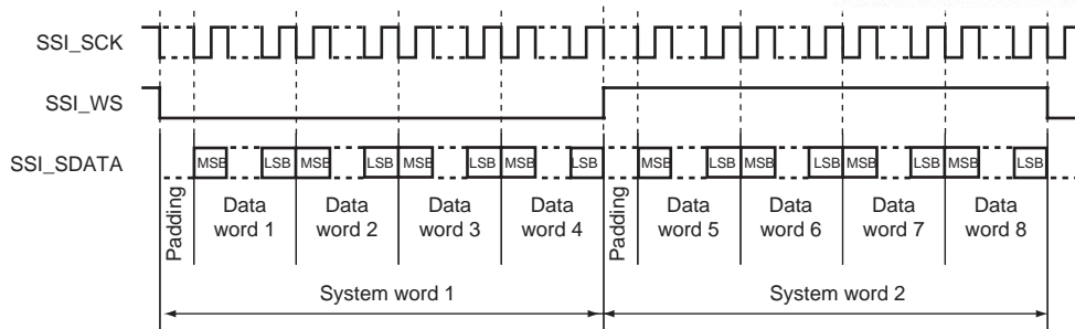
Figure 20.8 Multichannel Format (8 Channels, with Padding Bits First, Followed by Serial Data, with Padding)
