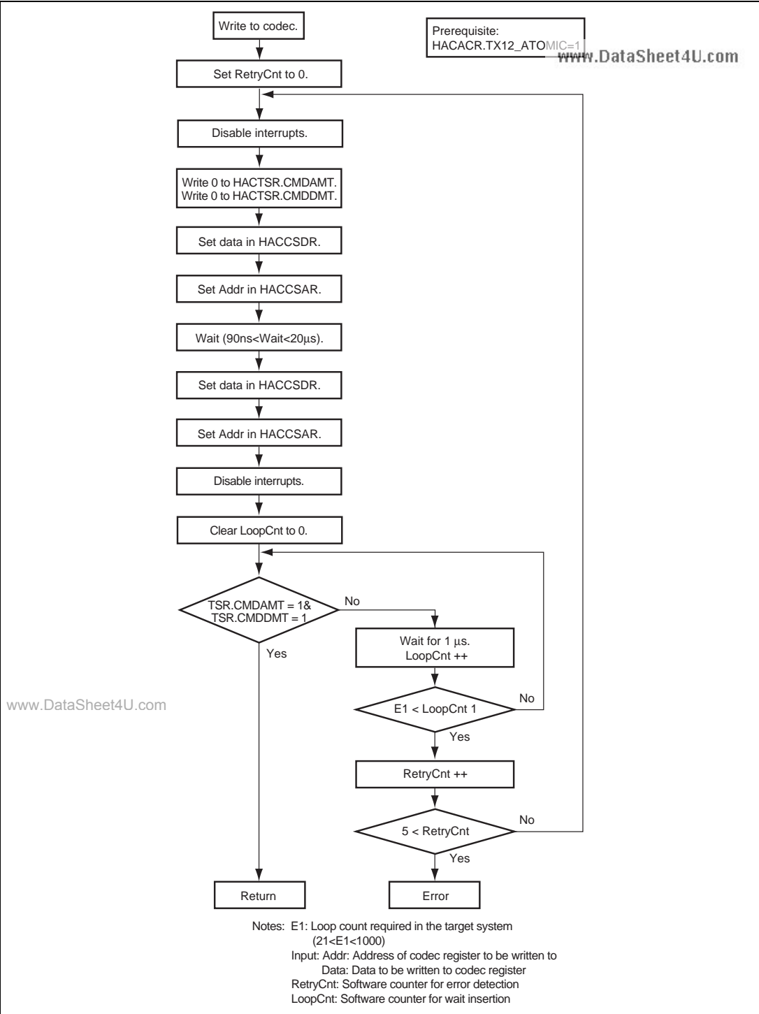
Figure 25.4 Sample Flowchart for Off-Chip Codec Register Write
