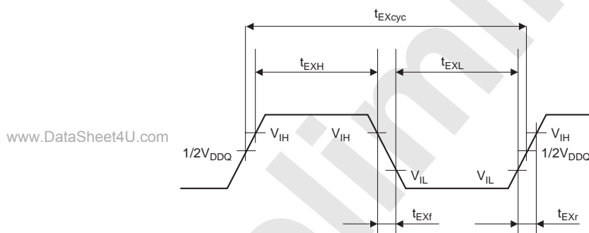
Figure 33.1 EXTAL Clock Input Timing
