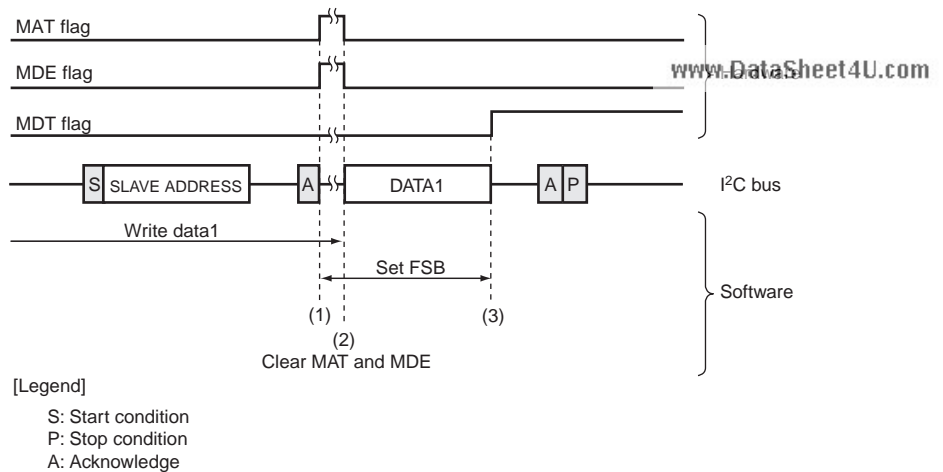
Figure 19.11 Operational Example of One-byte Data Transmission
