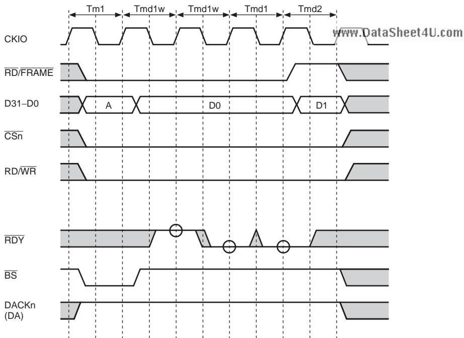
Figure 10.55 MPX Interface Timing 12 (Burst Write Cycle, AnW = 1, One External Wait Inserted, 32-Bit Bus Width, 64-Bit Data Transfer)
