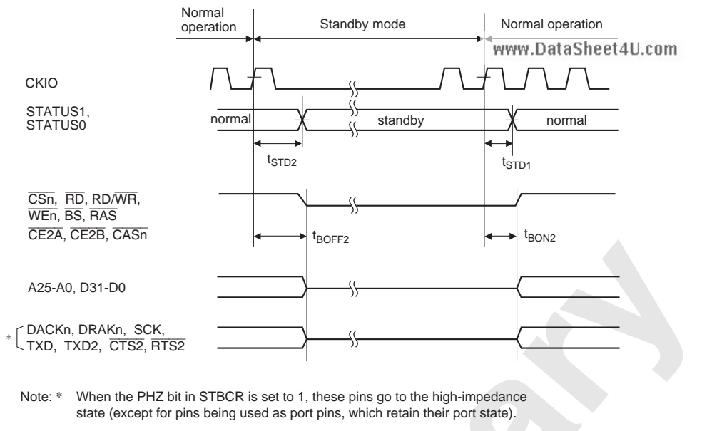
Figure 33.16 Pin Drive Timing for Standby Mode
