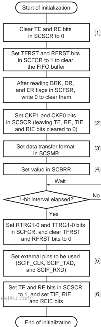
Figure 17.16 Sample SCIF Initialization Flowchart
