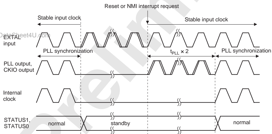
Figure 33.12 PLL Synchronization Settling Time in Case of \overline{RESET} , \overline{MRESET} or NMI Interrupt
