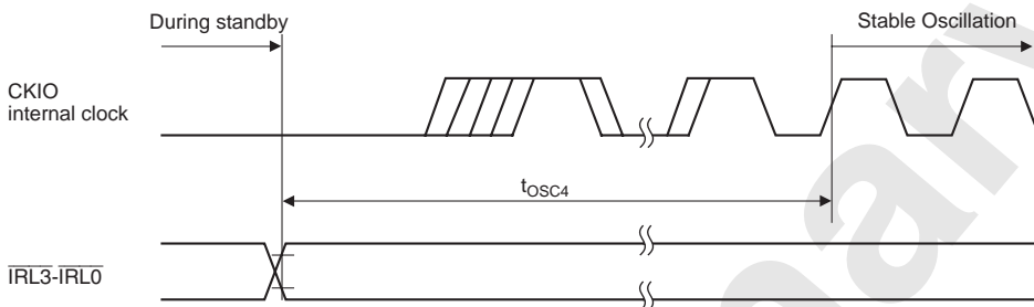
Figure 33.11 Standby Return Oscillation Settling Time (Return by \overline{IRL3} to \overline{IRL0} )
