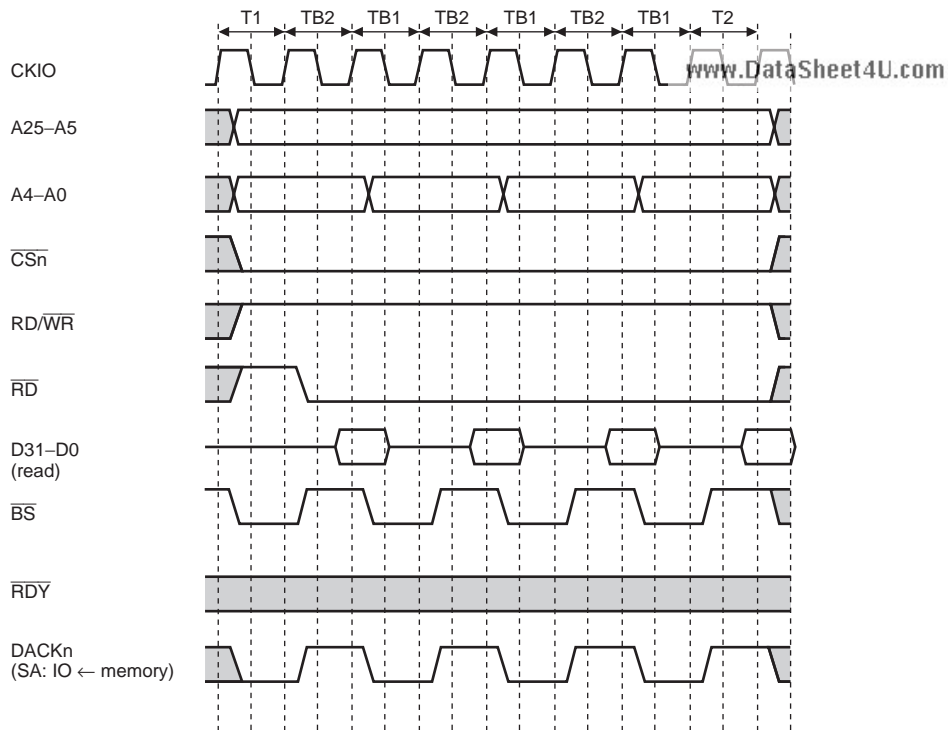
Figure 10.33 Burst ROM Basic Access Timing
