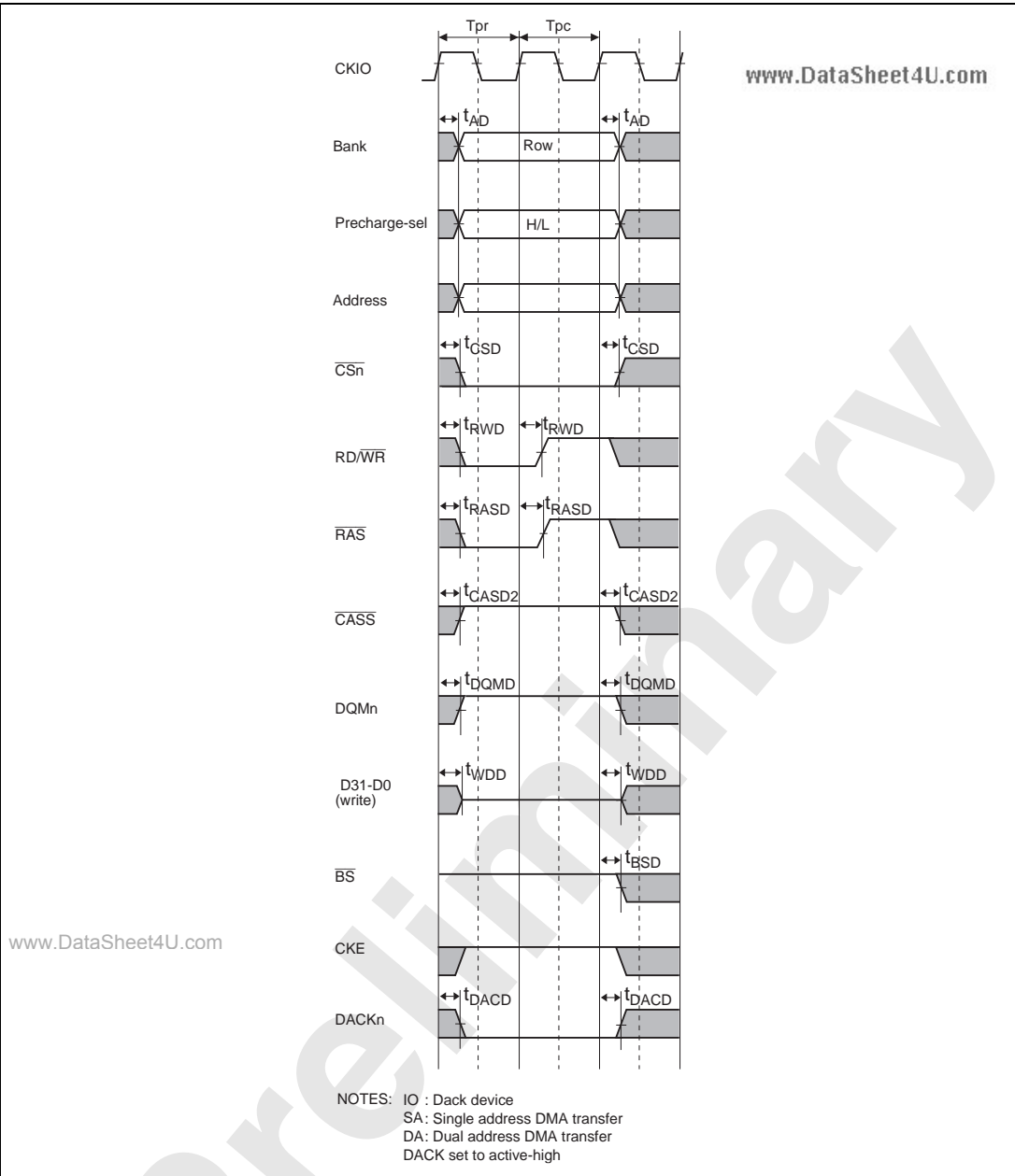
Figure 33.35 Synchronous DRAM Bus Cycle: Precharge Command (TPC[2:0]=001)
