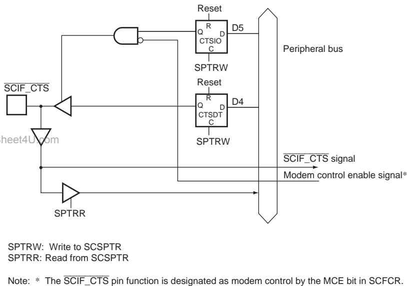
Figure 17.3 SCIF_CTS Pin (Only in Channels 1 and 2)
