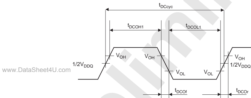
Figure 33.4 DCK Clock Output Timing (1)
