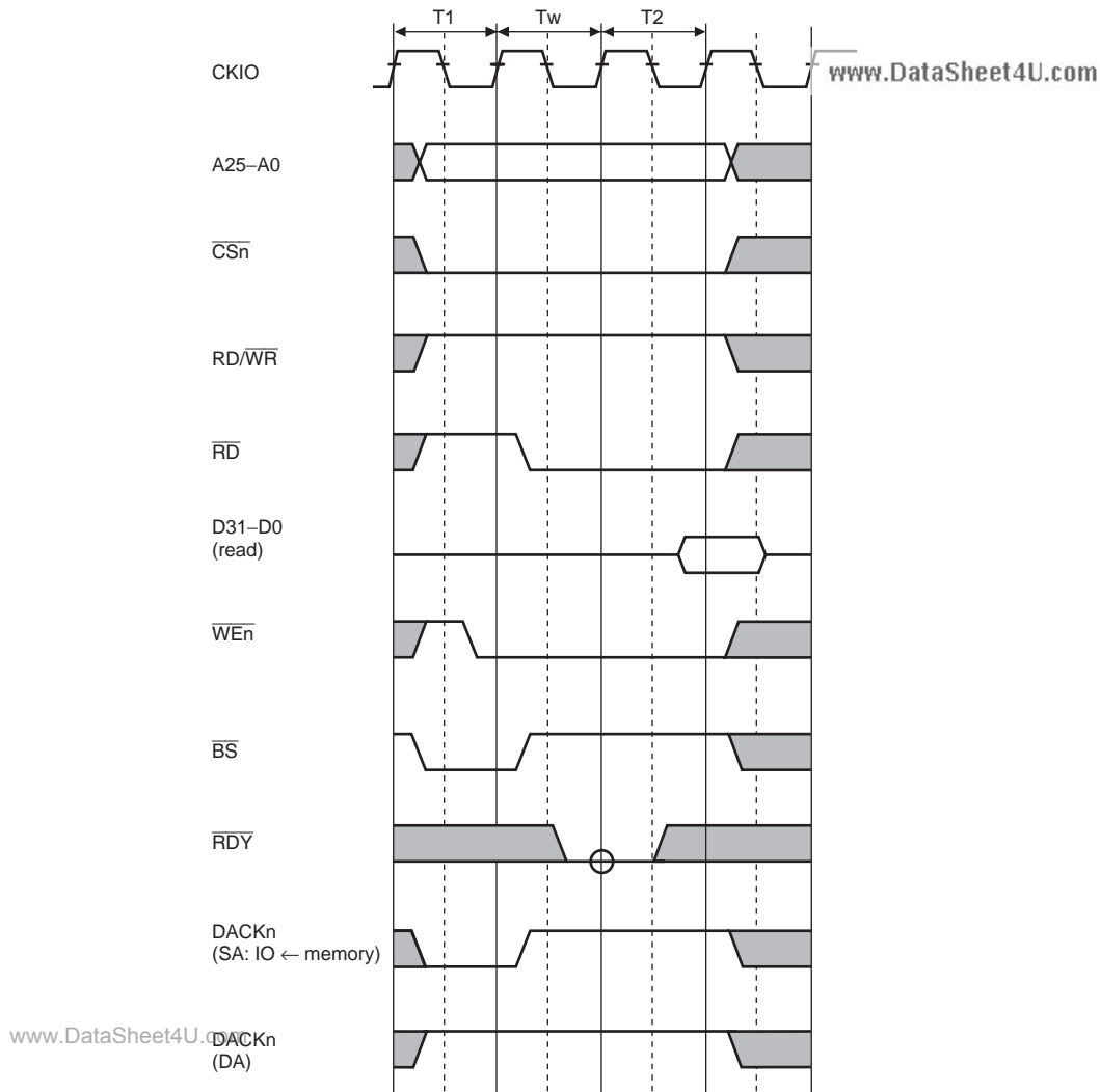
Figure 10.58 Byte Control SRAM Basic Read Cycle (One Internal Wait Cycle)
