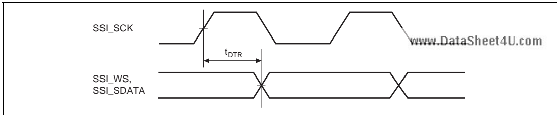
Figure 33.85 SSI Transmit Timing (1)
