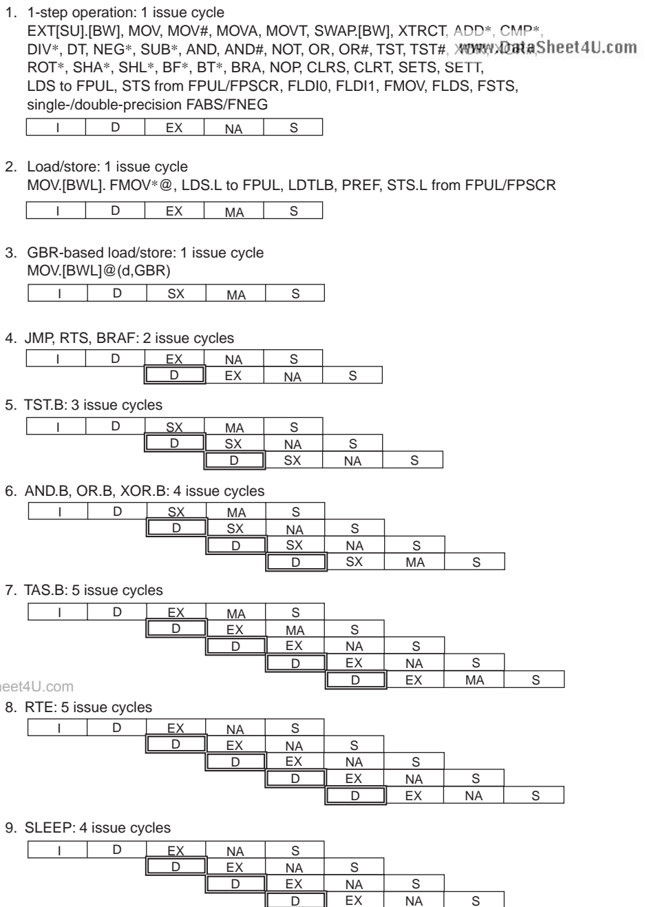
Figure 5.2 Instruction Execution Patterns
