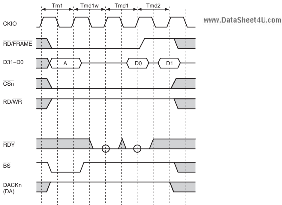
Figure 10.52 MPX Interface Timing 9 (Burst Read Cycle, AnW = 0, No External Wait, 32-Bit Bus Width, 64-Bit Data Transfer)
