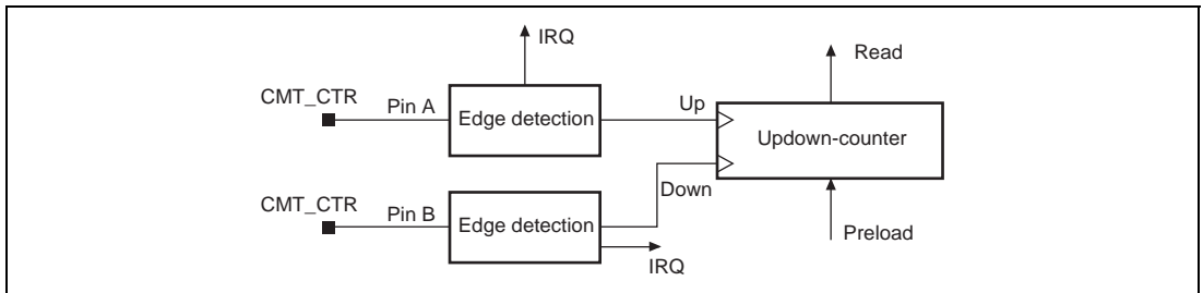
Figure 16.8 Updown-Counter Mode
