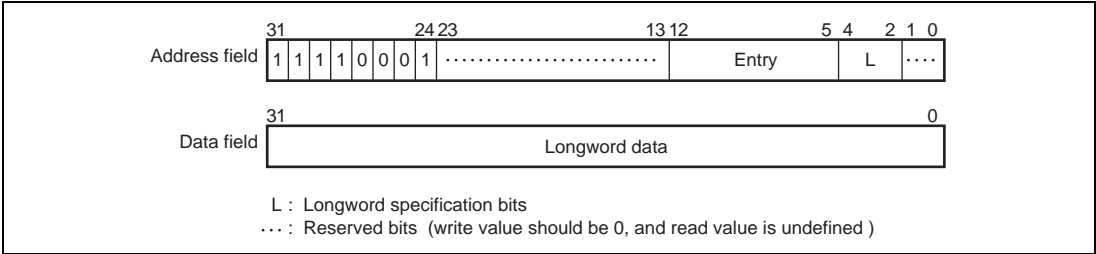
Figure 7.6 Memory-Mapped IC Data Array
