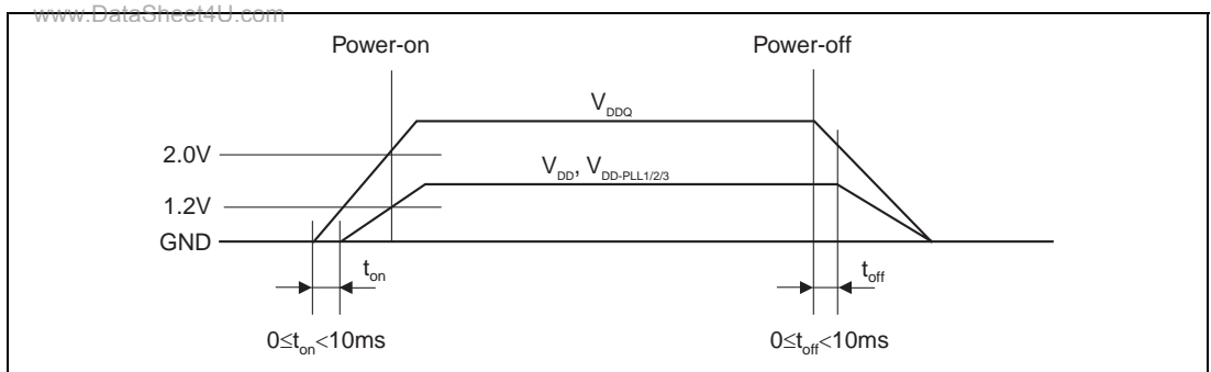
Figure F.1 Power-On and Power-Off Procedures
