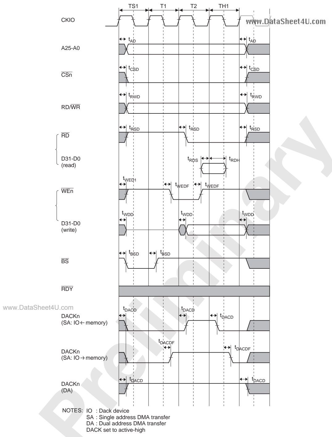
Figure 33.20 SRAM Bus Cycle: Basic Bus Cycle (No Wait, Address Setup/Hold Time Insertion, AnS=1, AnH=1)
