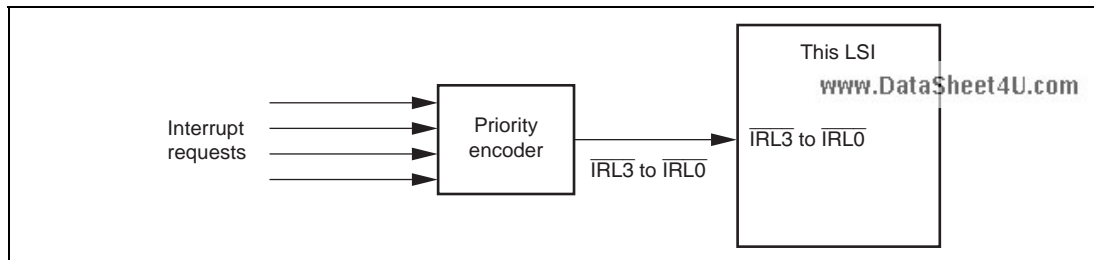
Figure 9.2 Example of IRL Interrupt Connection
