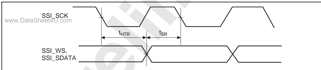
Figure 33.88 SSI Receive Timing (2)
