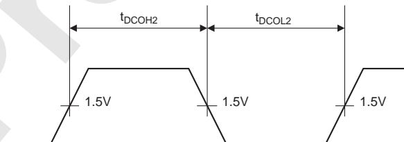
Figure 33.5 DCK Clock Output Timing (2)
