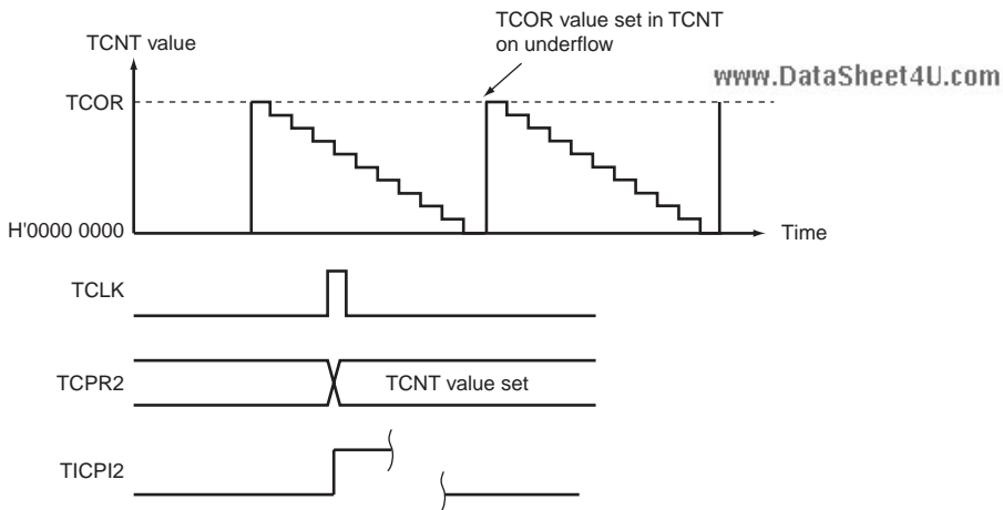
Figure 15.6 Operation Timing when Using Input Capture Function
