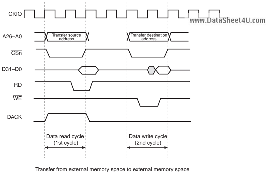
Figure 11.9 Example of Transfer Timing in Dual Address Mode
