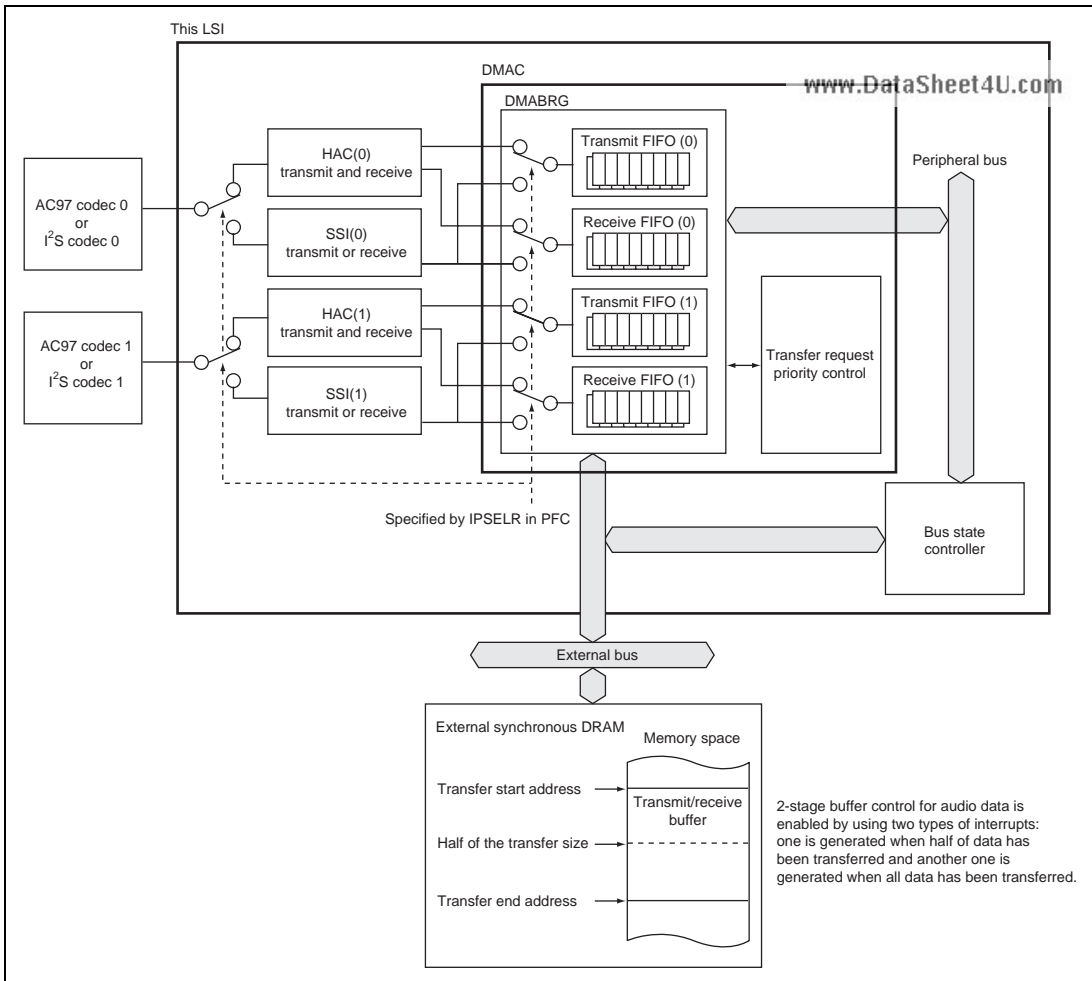
www.DataSheet4U.com Figure 11.31 Configuration of DMA for HAC/SSI
