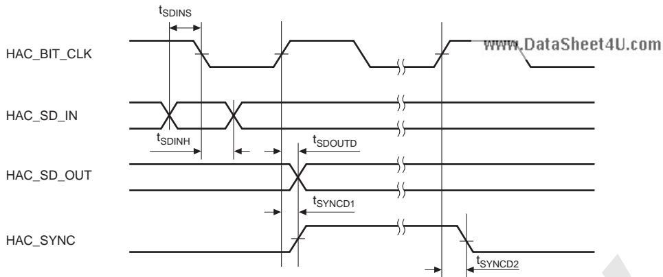
Figure 33.83 HAC Interface Module Signal Timing
