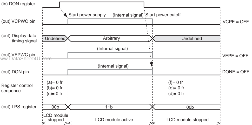
Figure 30.7 Power-Supply Control Sequence and States of the LCD Module
