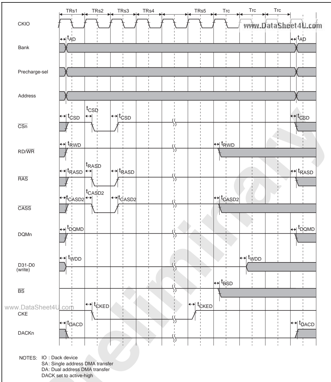
Figure 33.37 Synchronous DRAM Bus Cycle: Self-Refresh (TRC[2:0]=001)
