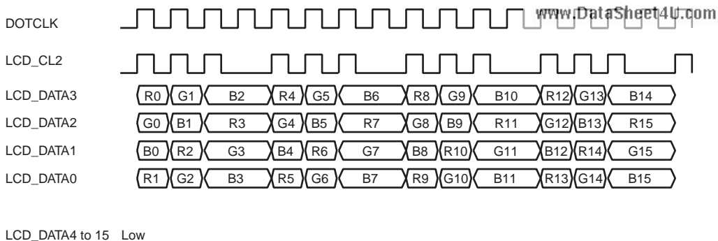
Figure 30.10 Clock and LCD Data Signal Example
