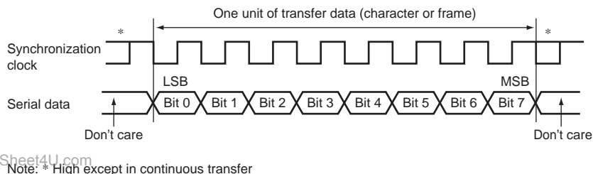
Figure 17.15 Data Format in Synchronous Communication
