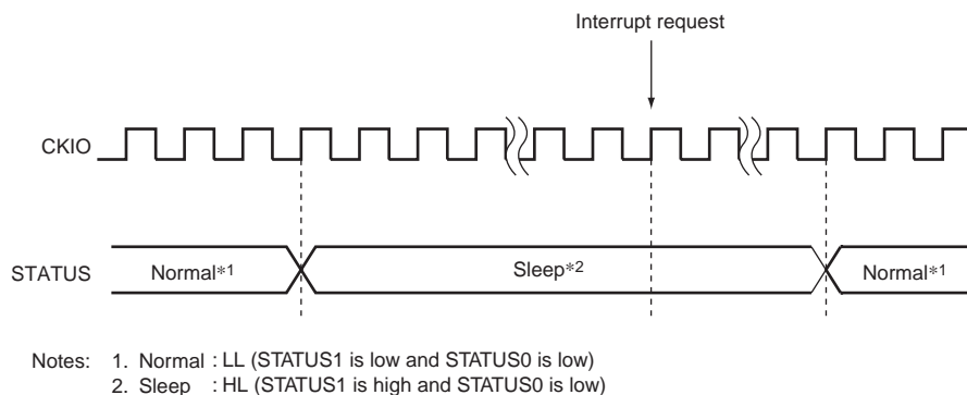
Figure 14.9 STATUS Output in Sequence of Deep Sleep → Interrupt
