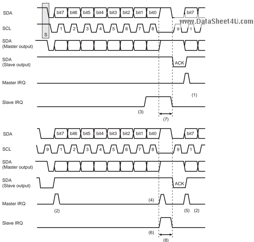
Figure 19.9 Data Transfer Mode Timing Chart
