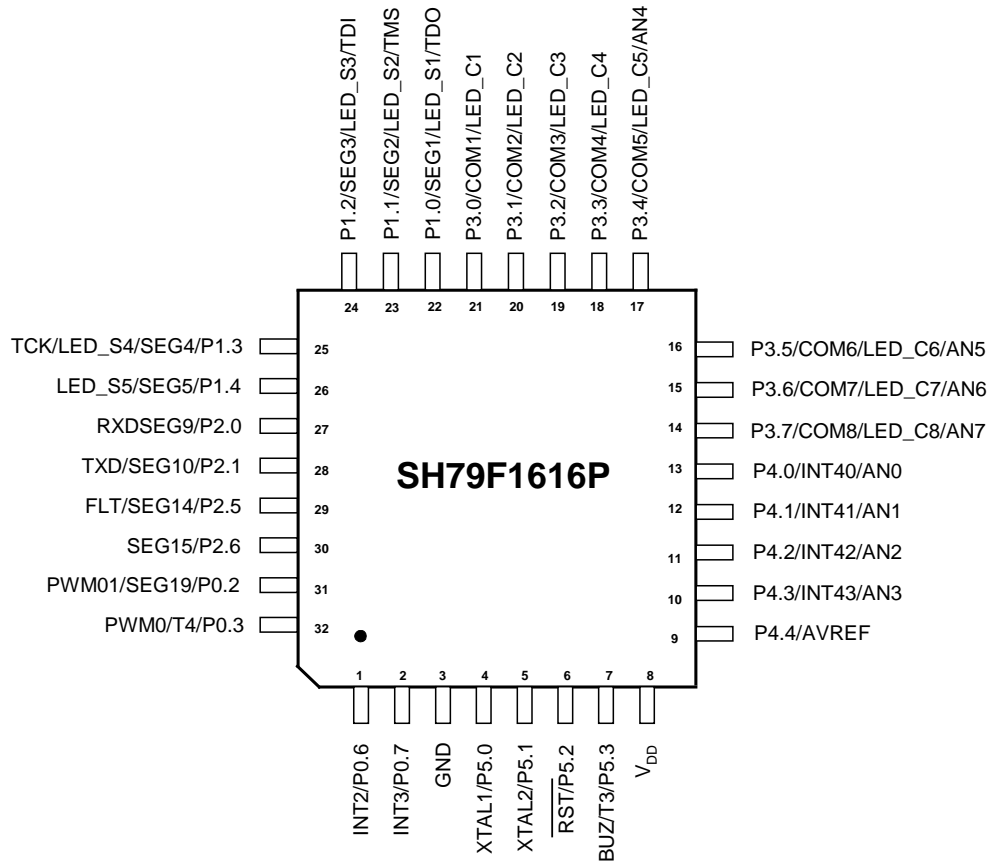
Pin Configuration Diagram
