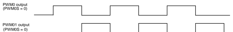
PWM0 and PWM01 pin output waveform
