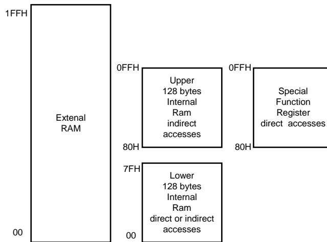
The Internal and External RAM Configuration
