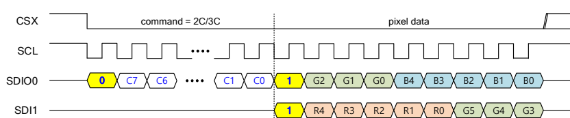
Figure 29 SPI 3-Wire 3553 Pixel Format
