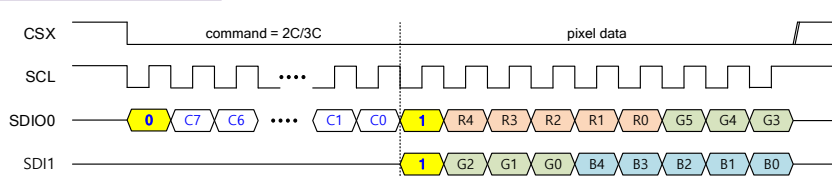
Figure 28 SPI 3-Wire 565 Pixel Format
