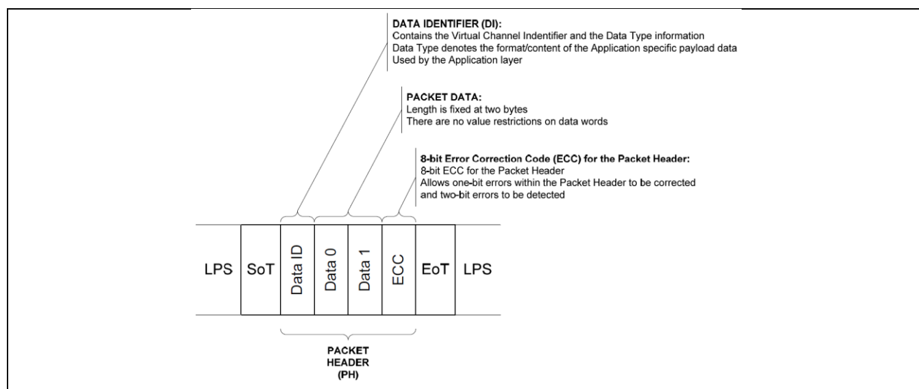
Figure 57 Short Packet Structure
