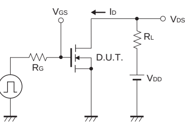
Fig.10 Switching Time Test Circuit
