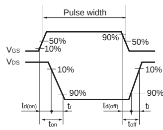
Fig.1-2 Switching Waveforms
