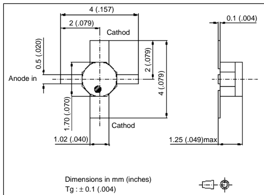
BH198 C_b=0.6\text{pF}
