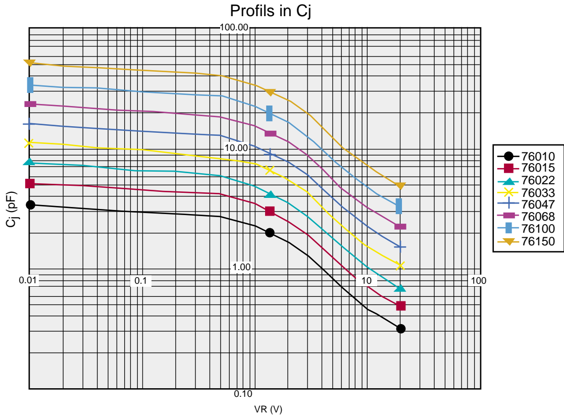
Typical junction capacitance versus reverse voltage
