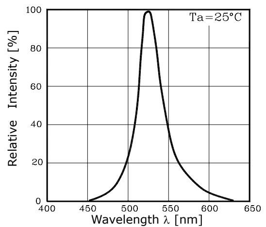
Fig. 4 Spectrum Distribution
