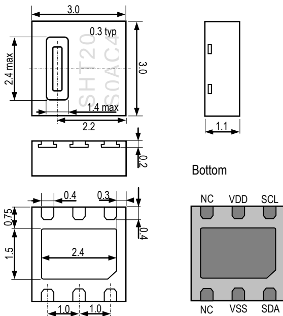
Figure 1: Drawing of SHT20S sensor package, dimensions are given in mm (1mm = 0.039inch), tolerances are \pm 0.1 mm. The die pad (center pad) is internally connected to VSS. The NC pads must be left floating. Numbering of E/O pads starts at lower right corner (indicated by notch in die pad) and goes clockwise (compare Table 2).
