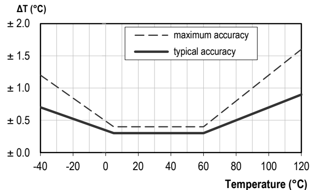
Figure 3 Typical and maximal temperature accuracy tolerance. For electronic impacts on accuracy please consult Sect. 5.3.
