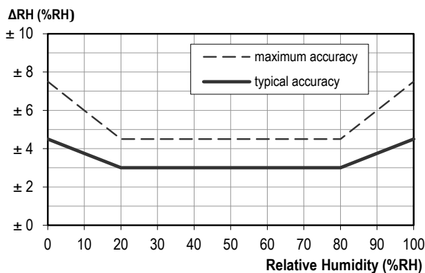
Figure 2 Typical and maximal tolerance at 25°C for relative humidity. For extensive information see Users Guide, Sect. 1.2. For electronic impacts on accuracy please consult Sect. 5.3.
