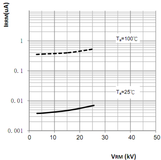
Reverse Characteristics
