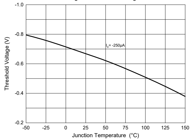
Fig. 6 - Threshold Voltage
