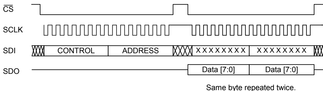
Figure 32. Register Read Operation via a 16-Bit SPI Port
