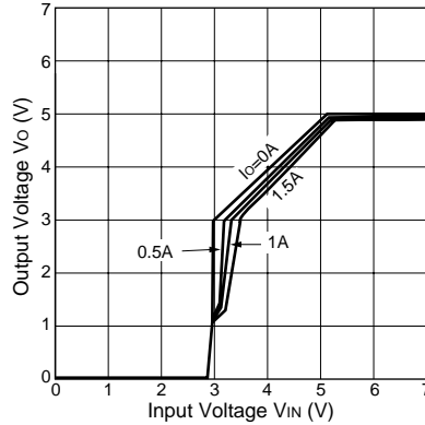
Output Voltage(SI-3050C)
