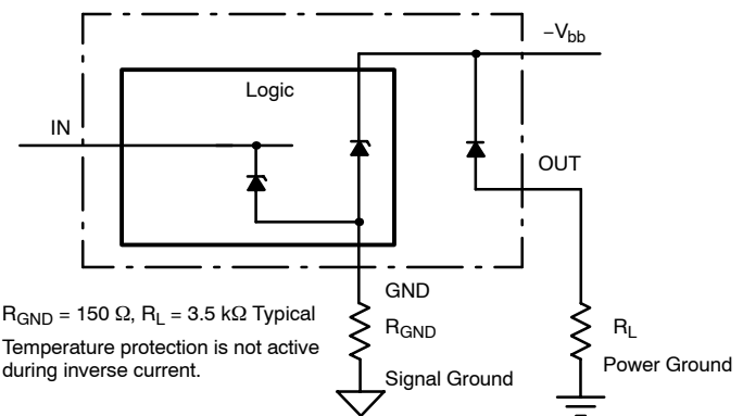
FIGURE 4. Reverse Pattern Protection
