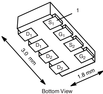
1206-8 ChipFET® (Dual)
