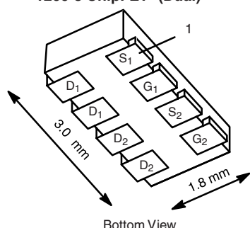
1206-8 ChipFET® (Dual)
