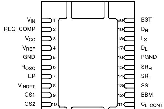
Si9122DLP (MLP65-20)
