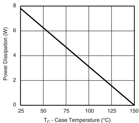
Power Derating
