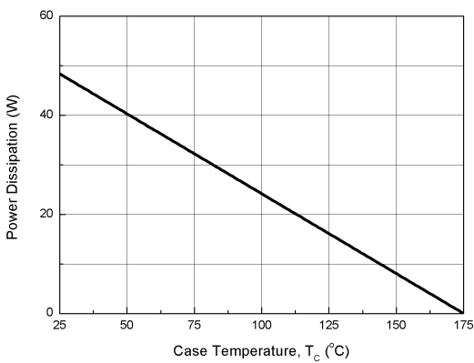
Fig. 5 Power Derating
