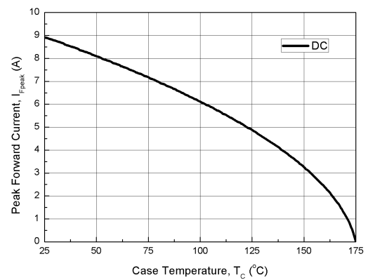
Fig. 6 Current Derating
