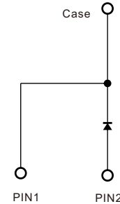
Inner Circuit
