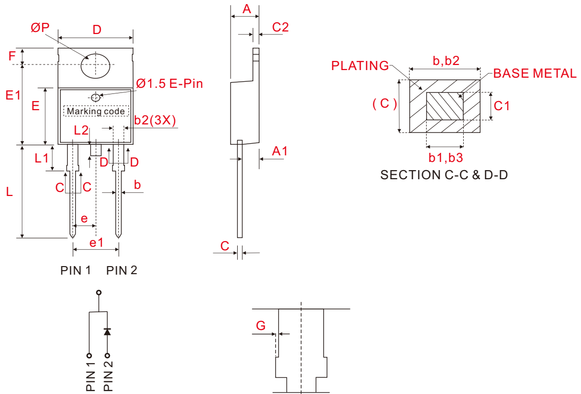
TO-220-2L
