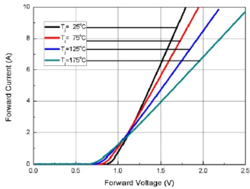
Fig. 1 Forward Characteristics
