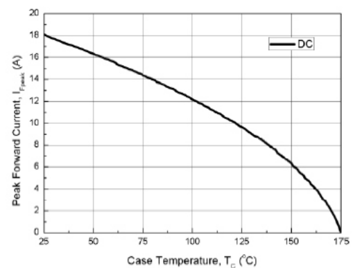
Fig. 6 Current Derating
