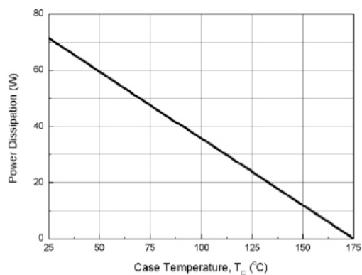
Fig. 5 Power Derating
