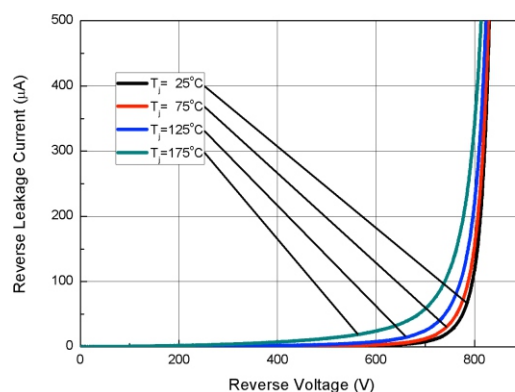
Fig. 2 Reverse Characteristics
