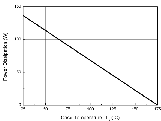
Fig. 5 Power Derating
