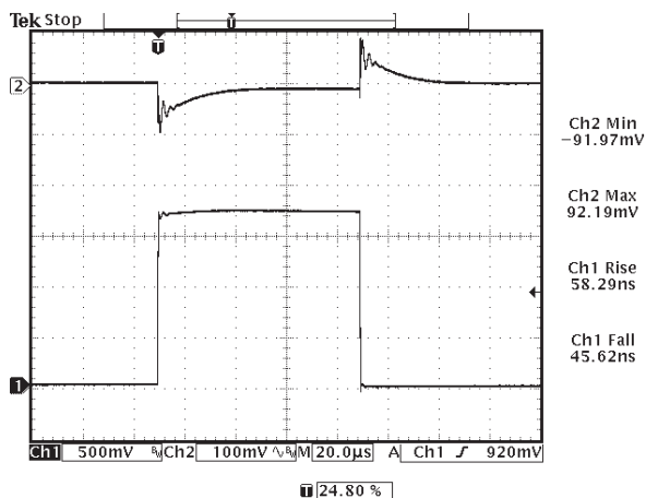
Figure 3 - Typical Transient Response, Vin = 12 V, Vout = 1.2 V Channel 1: 5 A Load Step, di/dt = 100 A/µs Channel 2: Deviation on Unit, Recovery Time = 10 µs
