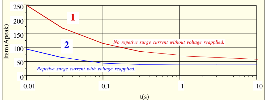
Fig.3 Surge current : I_{tsm} (\text{Apeak}) = f(t) for 25A models with I_{tsm} = 250\text{A}
