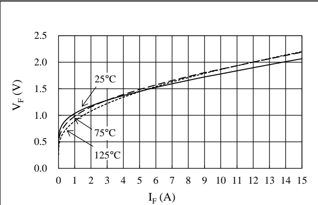
Figure 15-22. Freewheeling Diode V_F vs. I_F
