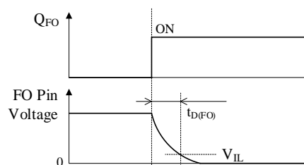
Figure 12-9. FO Pin Delay Time, t_{D(FO)}
