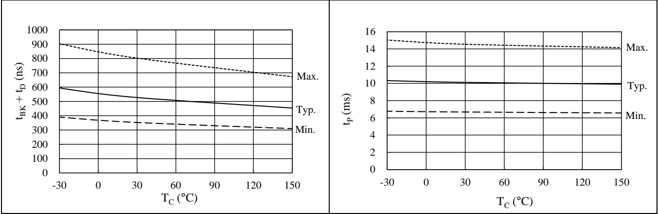
Figure 15-19. OCP Blanking Time, t_{BK(OC)} + Propagation Delay, t_{D(OC)} vs. T_C
