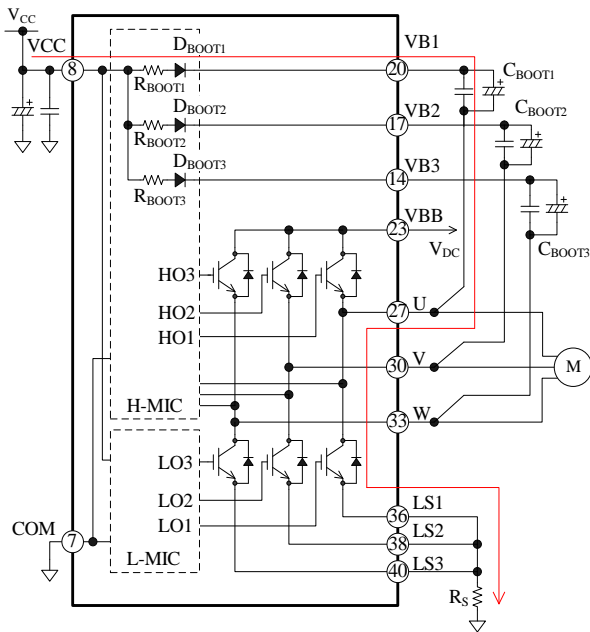
Figure 12-1. Bootstrap Circuit
