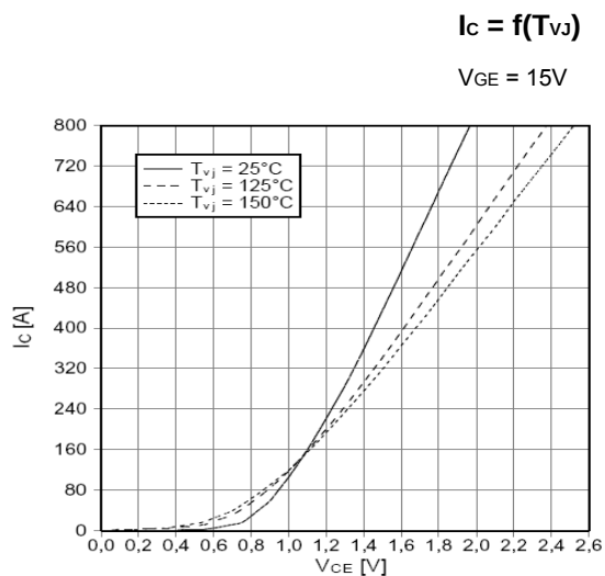
Fig.1, Output characteristic (typical)
