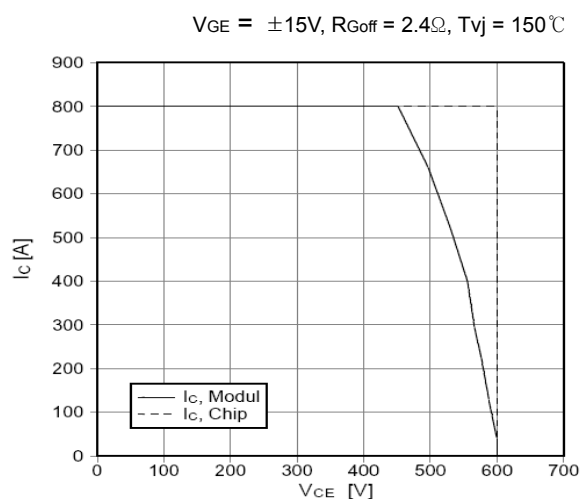
Fig.4, Reverse bias RBSOA
