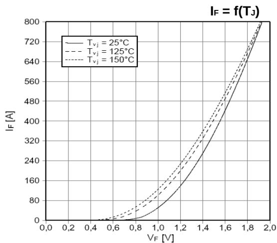
Fig.5, Forward characteristic of diode
