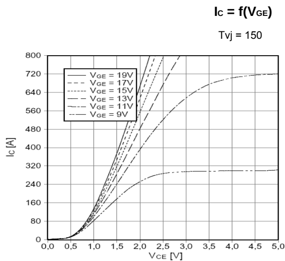
Fig.2 Output characteristic (typical)
