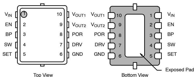
PowerPAK MLP33-10
