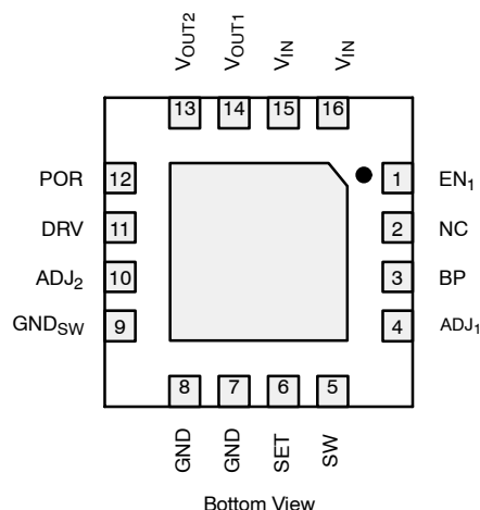
PowerPAK MLP44-16
