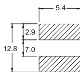
RECOMMENDED PAD
