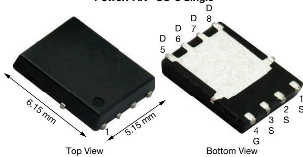
PowerPAK® SO-8 Single
