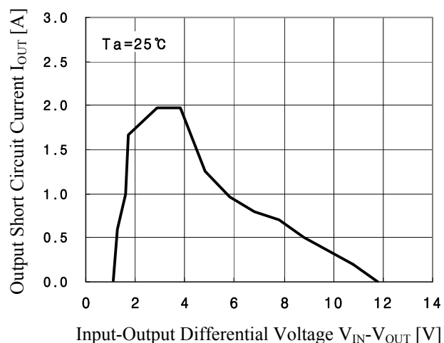
Fig.4 I_{OUT} vs V_{IN} - V_{OUT}
