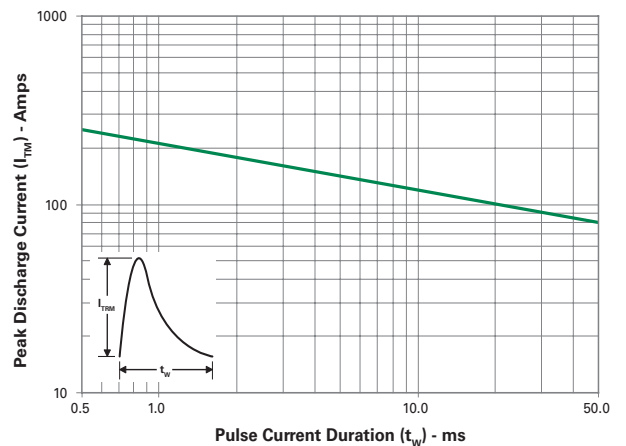
Figure 8: Peak Capacitor Discharge Current
