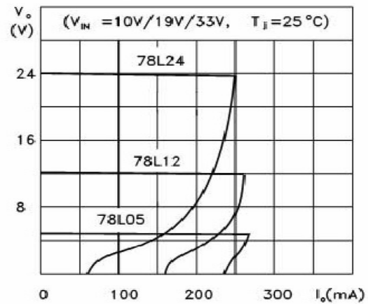
Load Characteristics
