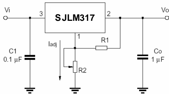
Fig.5 Programmable voltage regulator
