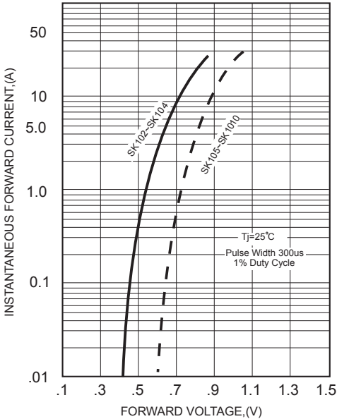
FIG.3-TYPICAL FORWARD CHARACTERISTICS
