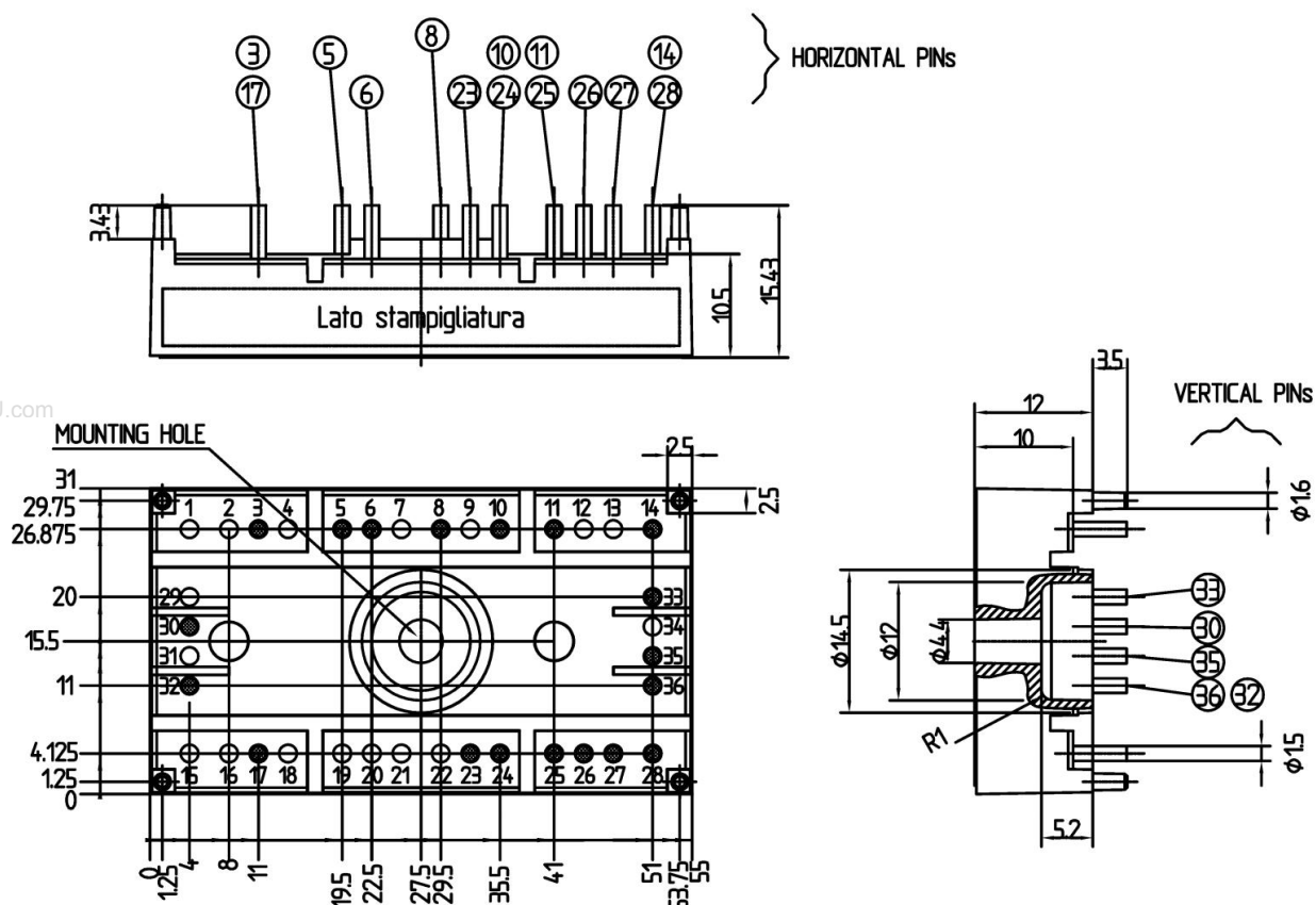
Case T 61 (Suggested hole diameter, in the PCB, for solder pins and plastic mounting pins: 2mm)
