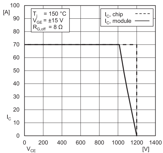
Fig. 13: IGBT Reverse Bias Safe Operating Area (RBSOA)
