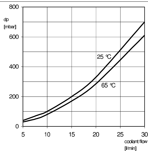
Fig. 7: Pressure drop characteristic
