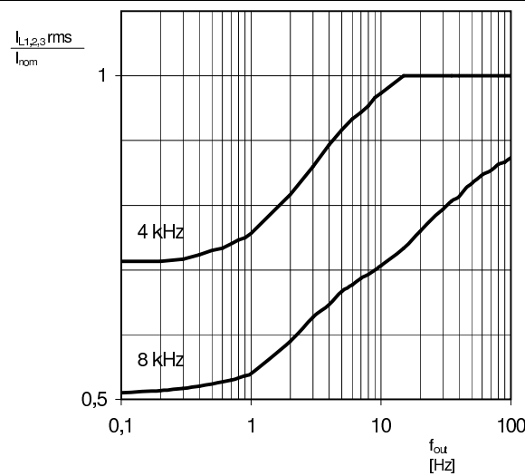
Fig. 11: Normalized output current vs. output frequency
