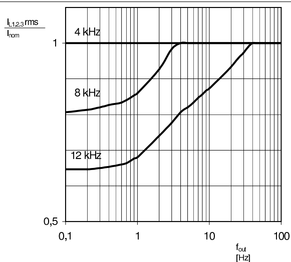
Fig. 9: Normalized output current vs. output frequency
