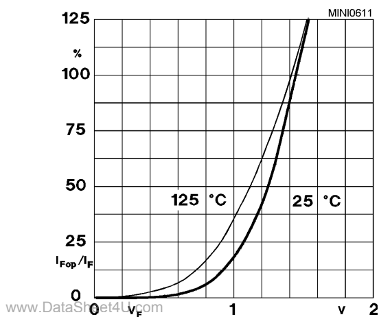
Fig. 11 Typ. freewheeling diode forward characteristic
