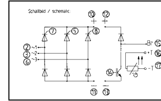
Circuit AHB
