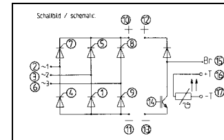
Circuit ATB
