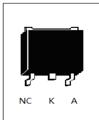
TO-252AA
