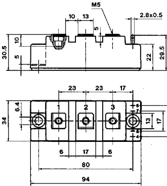
Cases D 56 ... 58 SEMITRANS® 3 L = 2 x 28 mm Low Inductance L_{CE} < 20 nH
