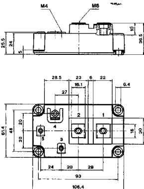
Cases D 59 ... 60 SEMITRANS® 4 Low Inductance L_{CE} < 20 nH
