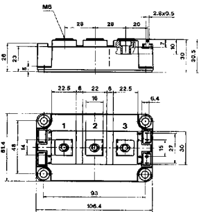
Cases D 59 ... 60 SEMITRANS® 4 Low Inductance L_{CE} < 20 nH
