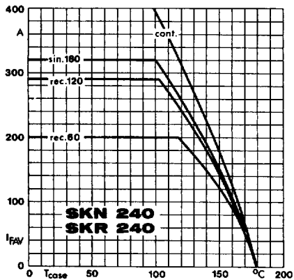
Fig. 3 c Rated forward current vs. case temperature
