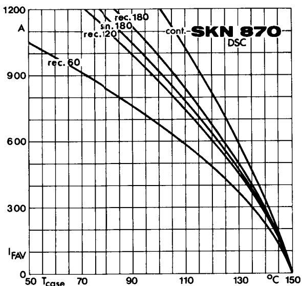
Fig. 3 e Rated forward current vs. case temperature
