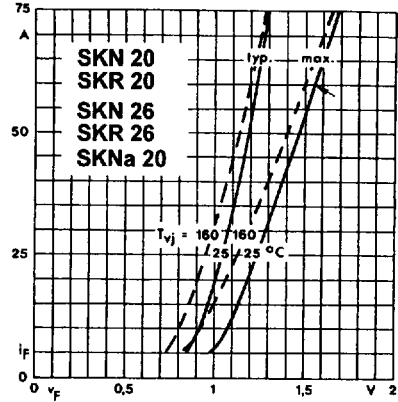
Fig. 6 Forward characteristics
