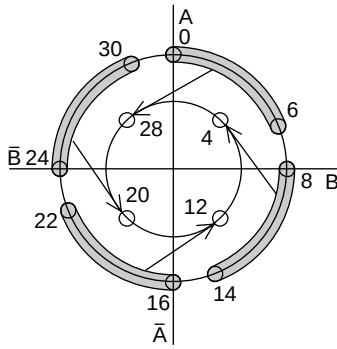
1-2 phase → 2 phase
