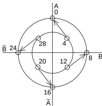
2 phase → 1-2 phase
