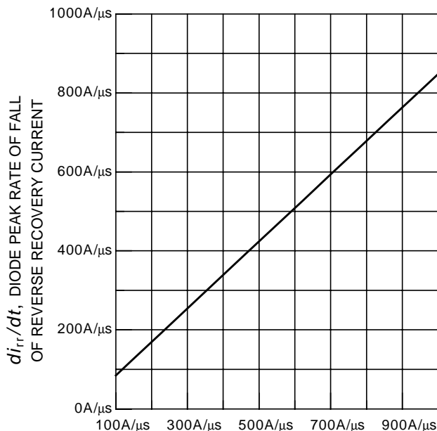
di_F/dt , DIODE CURRENT SLOPE Figure 24. Typical diode peak rate of fall of reverse recovery current as a function of diode current slope ( V_R = 200V , T_j = 125^\circ C )
